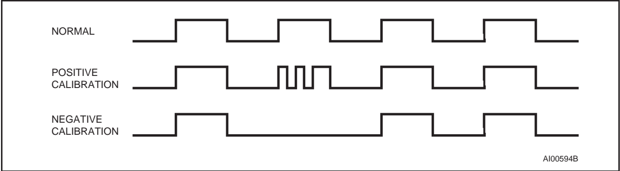
Figure 19. Clock Calibration
