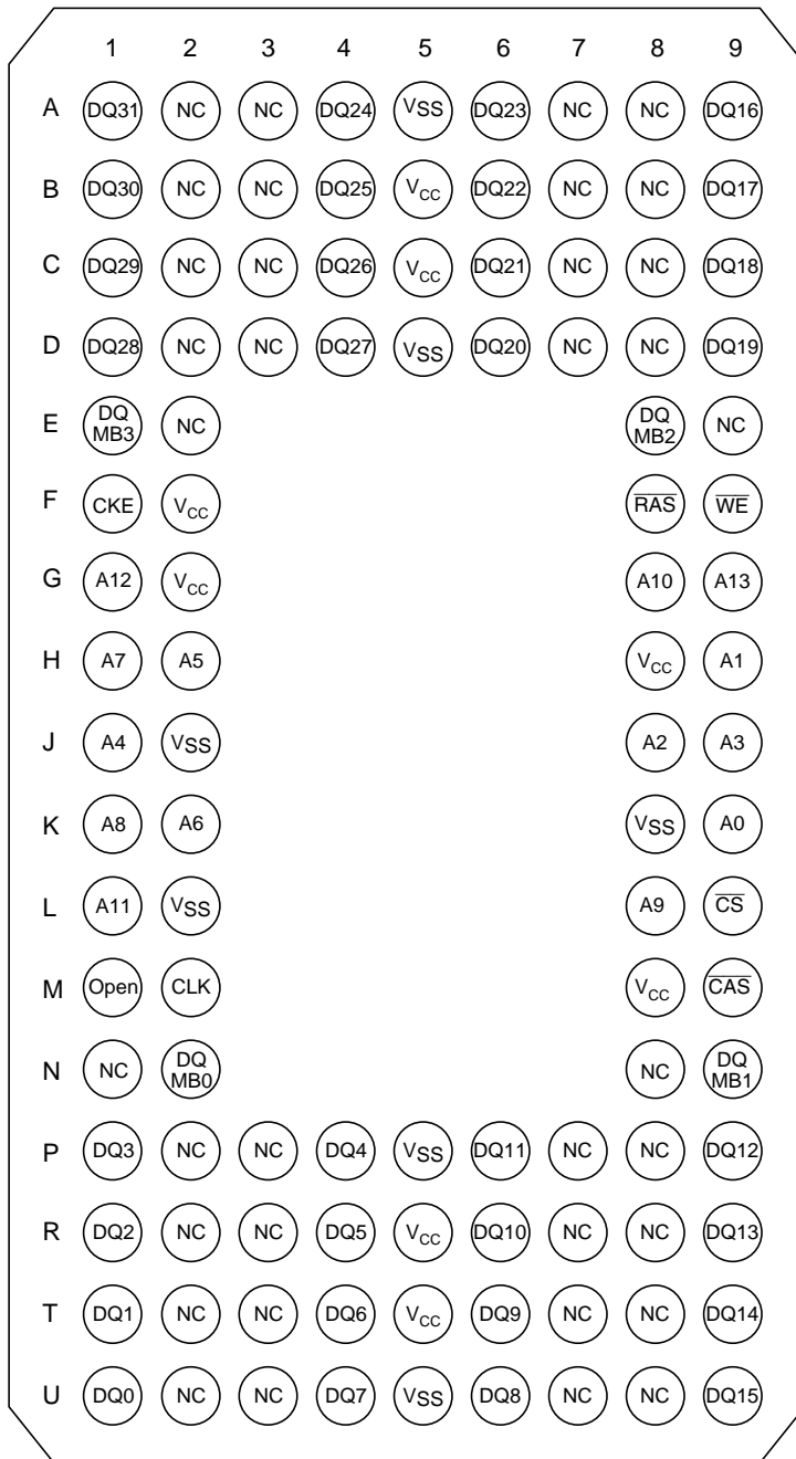
(Top view)
