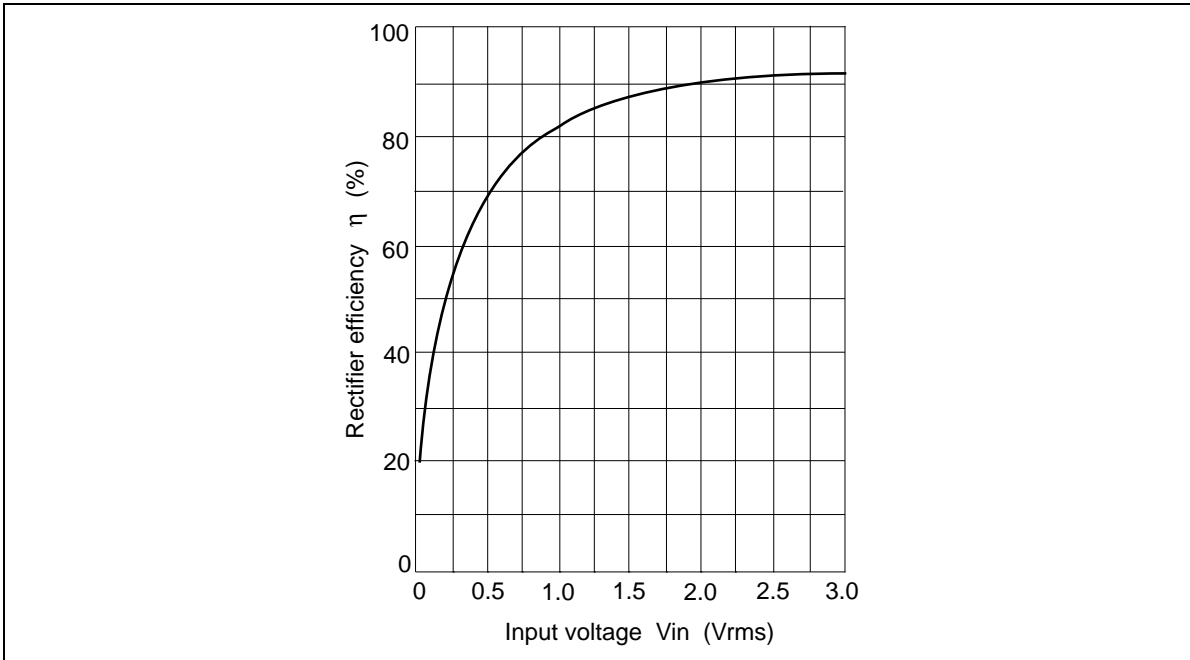
Fig.4 Rectifier efficiency Vs. Input voltage
