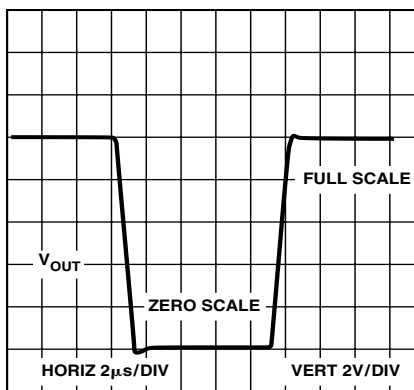
Figure 8. Large Signal Pulse Response
