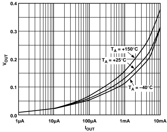
Figure 9. V_{OUT} vs. I_{OUT} ( V_{OUT} = \text{LOW} )
