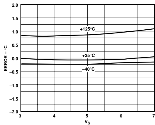
Figure 7. Setpoint Error vs. Supply Voltage
