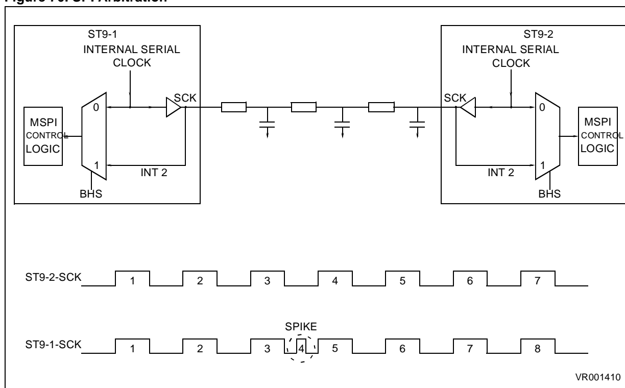
Figure 70. SPI Arbitration
