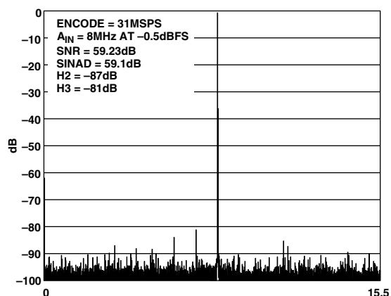
TPC 7. FFT: FS = 31 MSPS, A_{IN} = 8\text{ MHz @ } -0.5\text{ dBFS} , Differential, 1 V p-p Input Range
