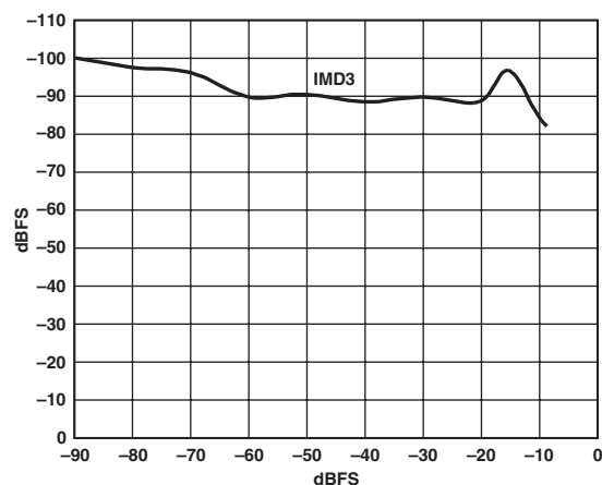
TPC 30. Third Order IMD vs. AIN Level, f_S = 105 MSPS, f_{IN} = 150.3 and 151.3 MHz, Differential AIN, SFDR Enabled
