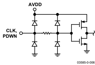
Figure 7. Equivalent Digital Input Circuit
