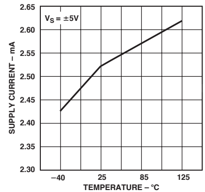
TPC 9. Supply Current vs. Temperature at \pm 5 V
