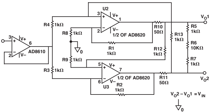
Figure 30. Differential Driver
