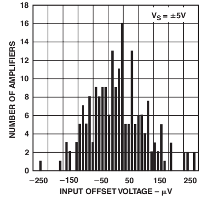
TPC 3. Input Offset Voltage at \pm 5 V
