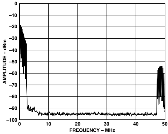
Figure 44. AD9777, Real DAC Output of Complex Input Signal Near Baseband (Positive Frequencies Only), Interpolation = 4x, No Modulation in AD9777
