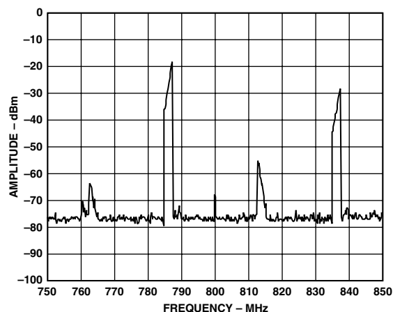
Figure 50. AD9777, Real DAC Output of Complex Input Signal Near Baseband (Positive Frequencies Only), Interpolation = 8\times , Complex Modulation in AD9777 = +f_{DAC}/8
