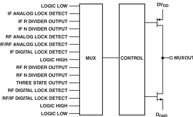
Figure 7. MUXOUT Circuit
