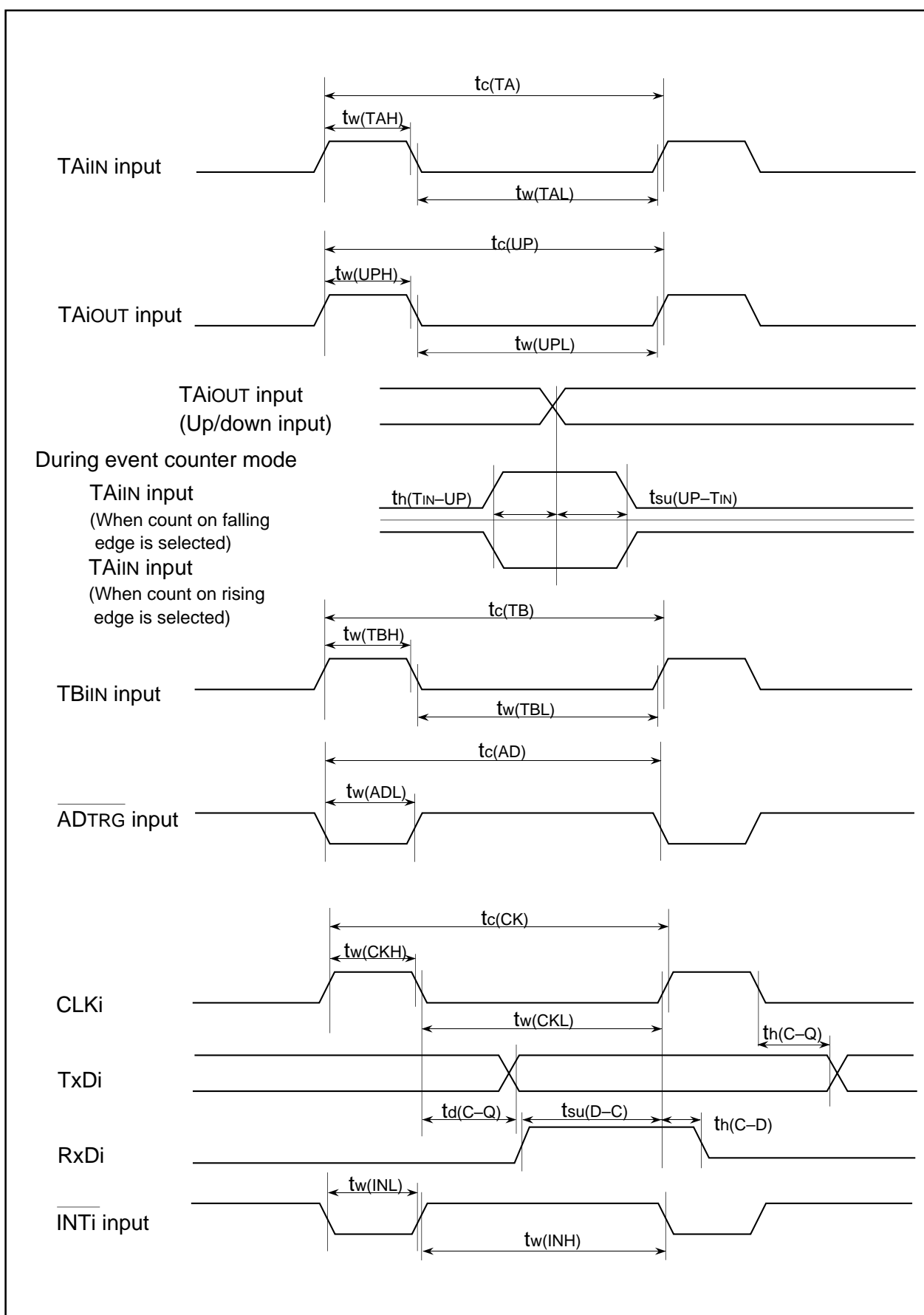
Figure 1.20.1. Timing diagram
