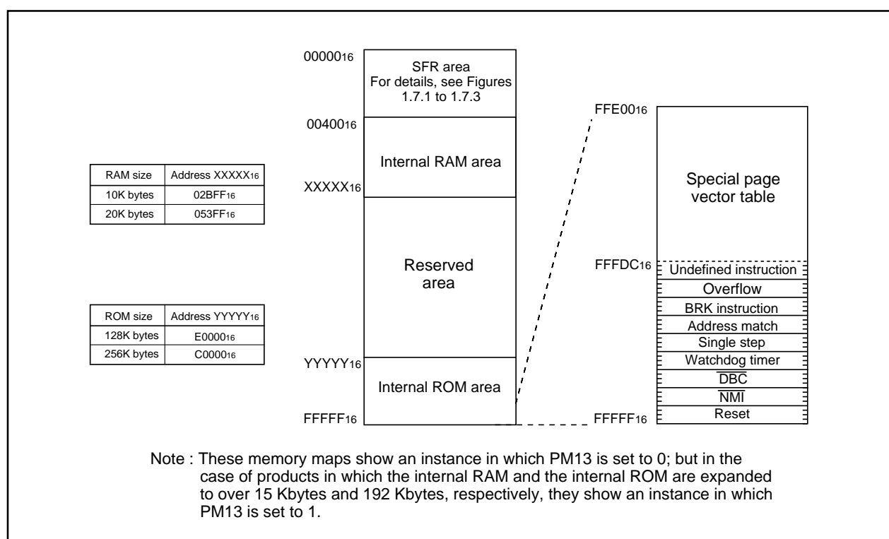
Figure 1.4.1. Memory map
