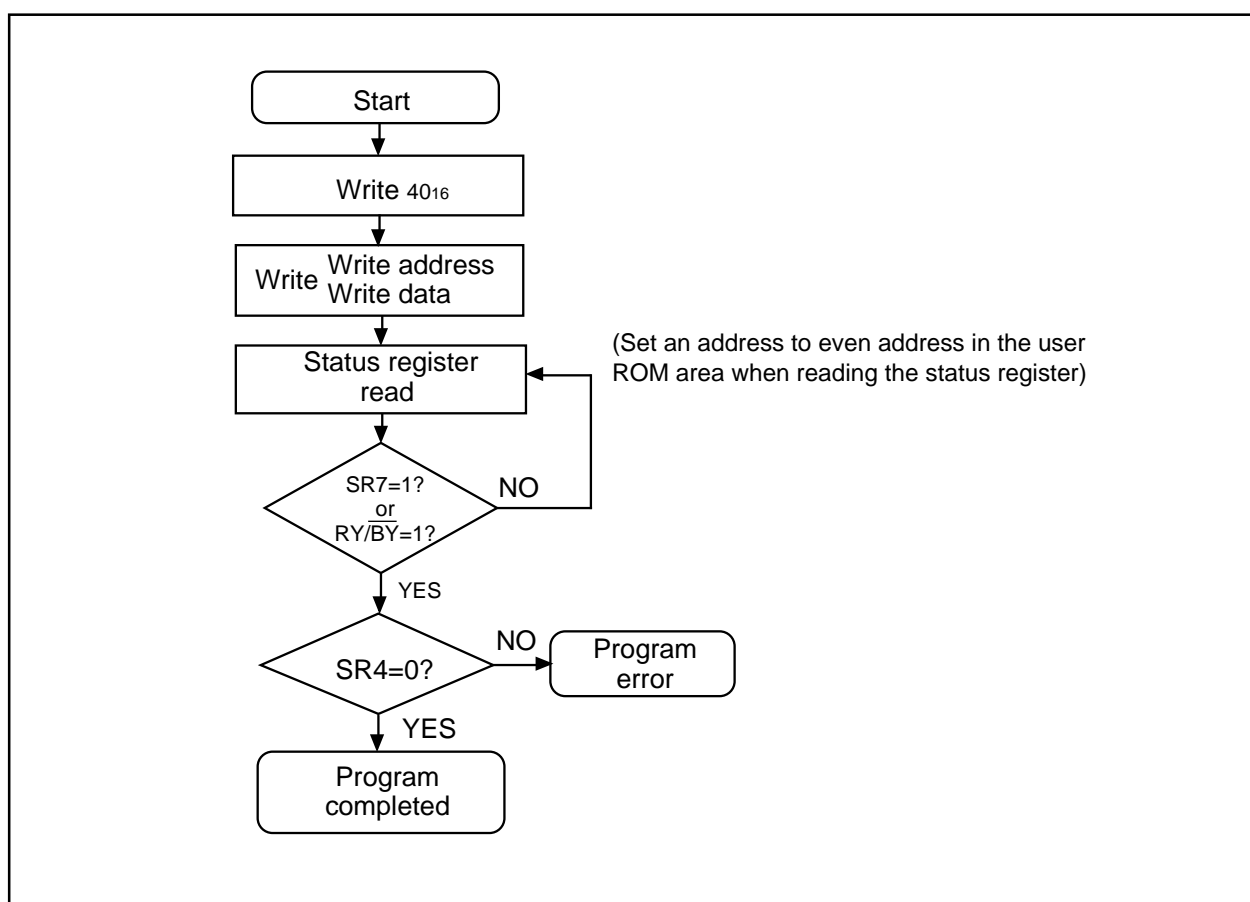
Figure 1.29.3. Program flowchart
