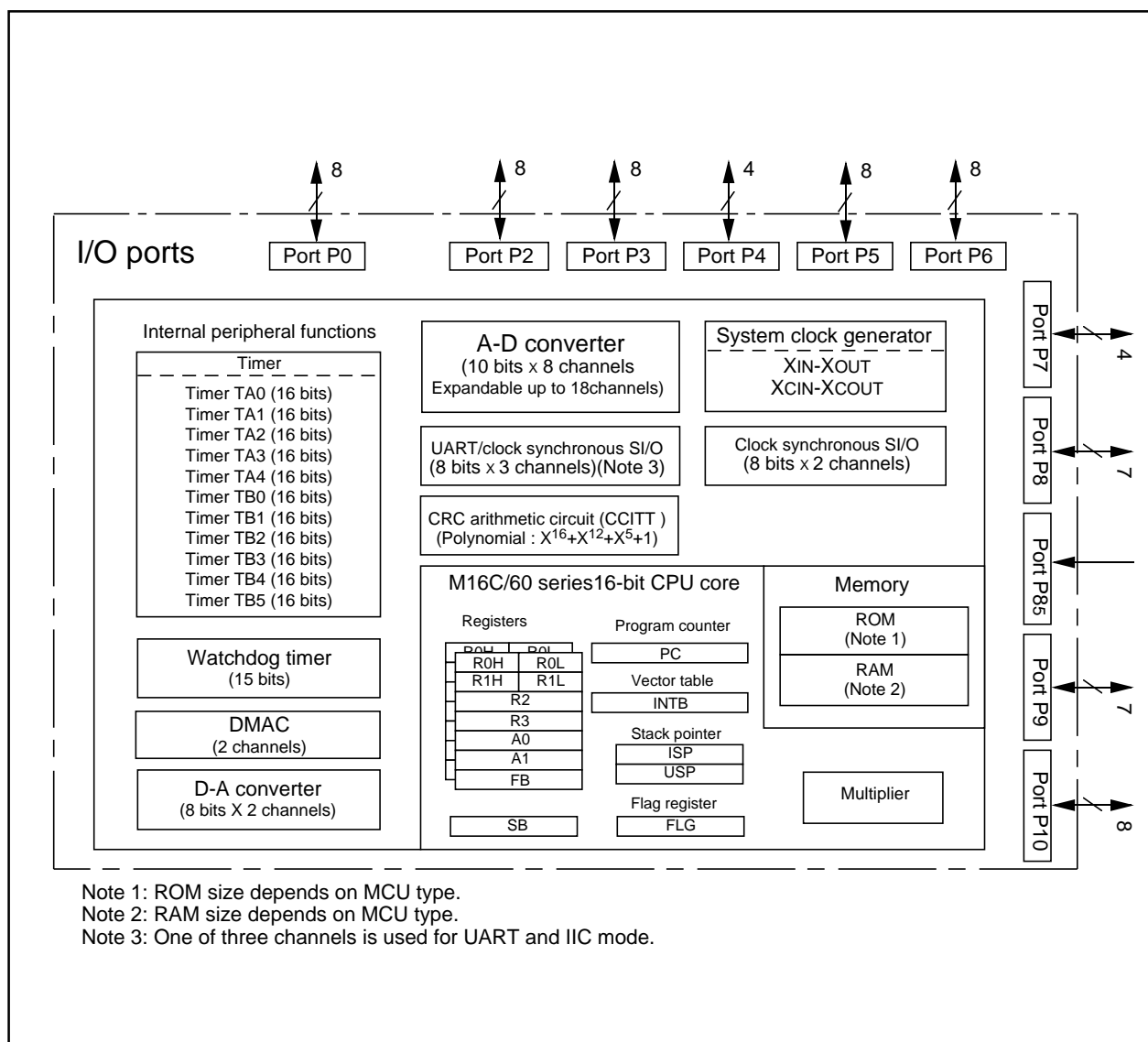
Figure 1.1.2. Block diagram of M16C/62N (80-pin version) group
