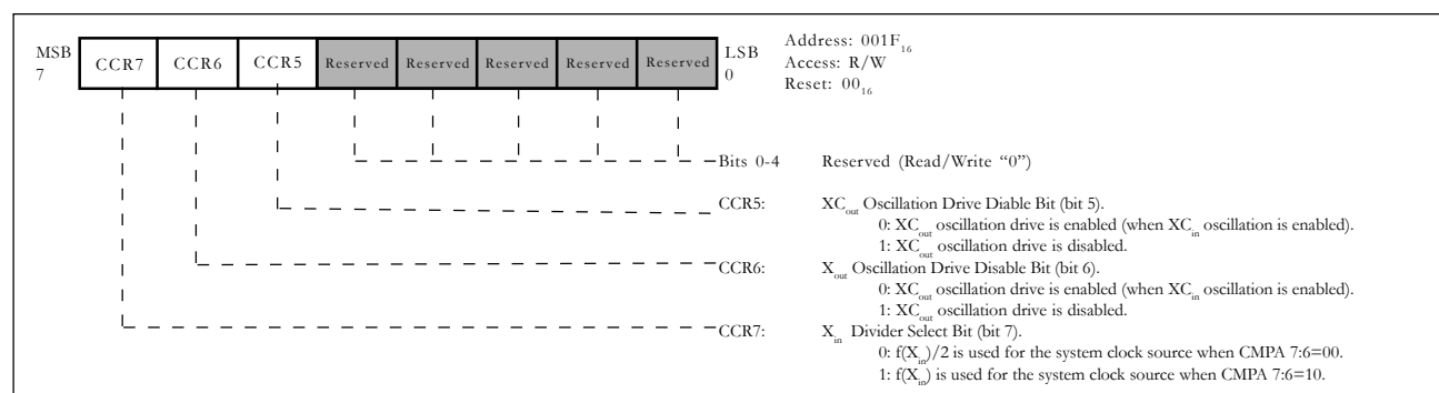
Fig. 1.89. Clock Control Register (CCR)
