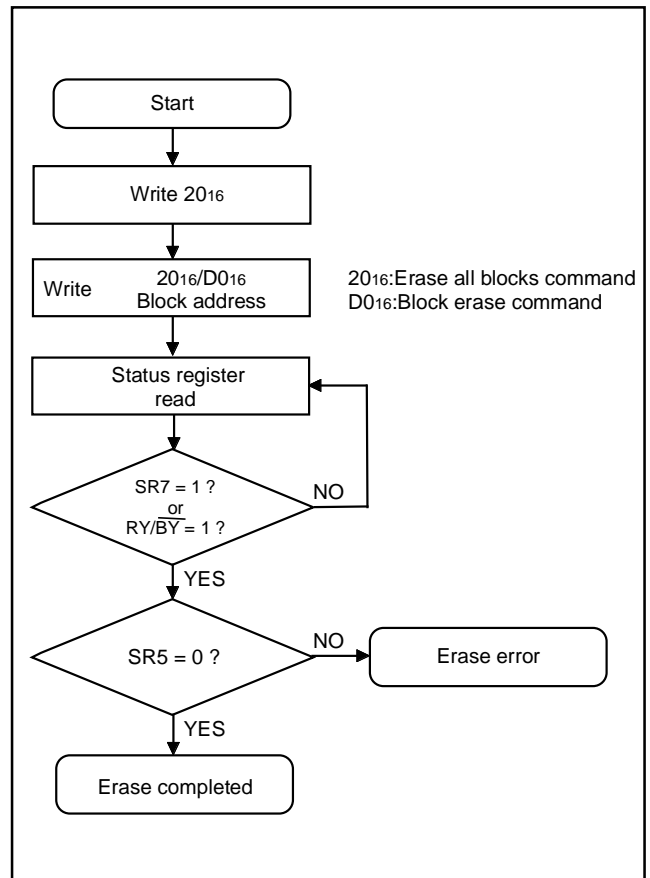
Fig. 92 Erase flowchart
