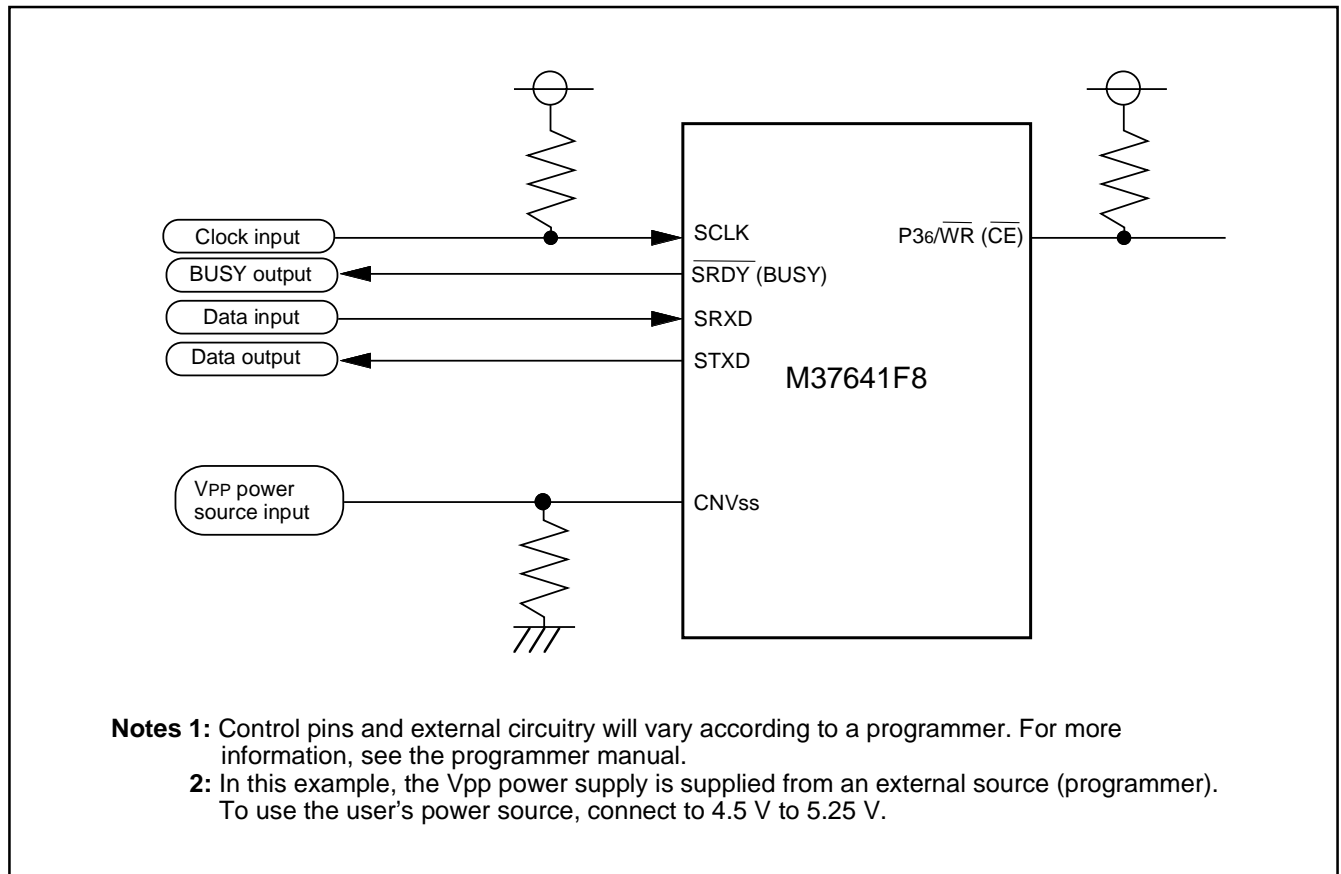
Fig. 110 Example circuit application for standard serial I/O mode
