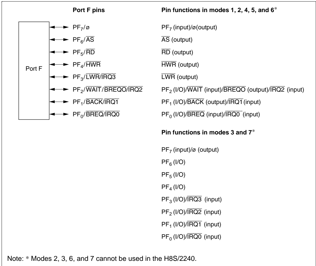
Figure 8-24 Port F Pin Functions
