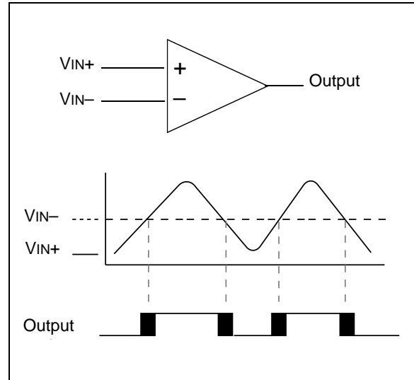
FIGURE 7-2: SINGLE COMPARATOR
