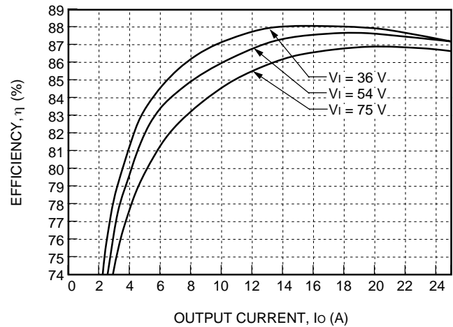
Figure 3. Typical FW300B1 Efficiency vs. Output Current at Room Temperature
