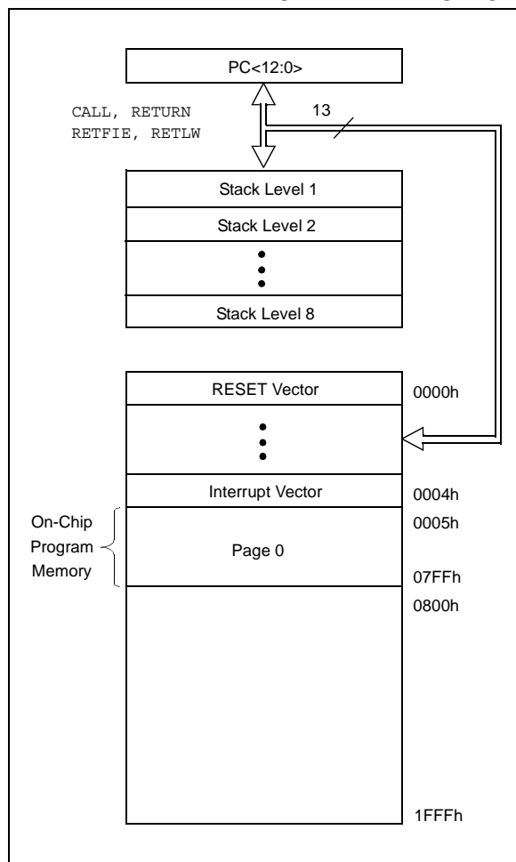
FIGURE 2-1: PIC16F870/871 PROGRAM MEMORY MAP AND STACK
