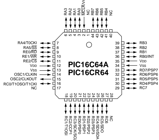
PLCC
