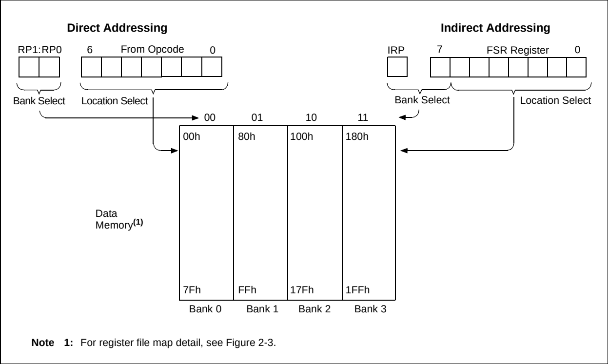
FIGURE 2-5: DIRECT/INDIRECT ADDRESSING
