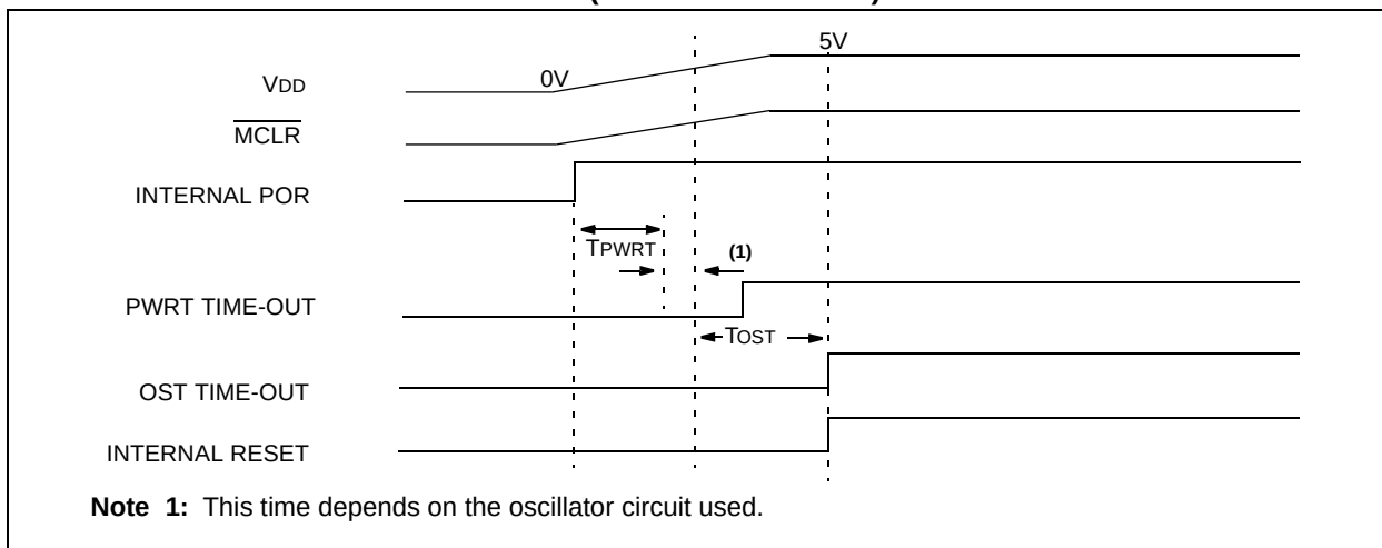
FIGURE 14-9: SLOW V_{DD} RISE TIME ( \overline{\text{MCLR}} TIED TO V_{DD} )
