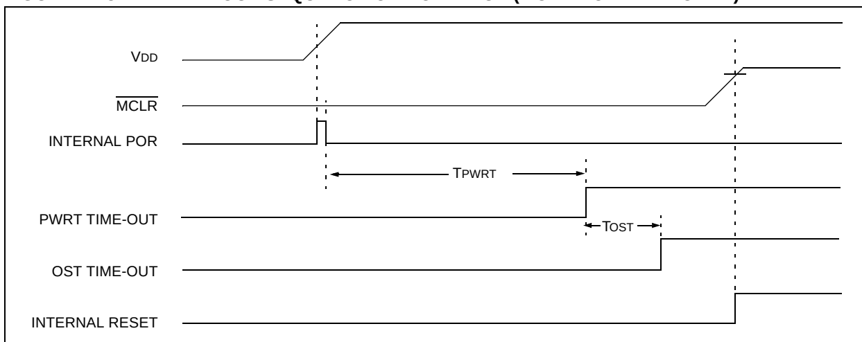
FIGURE 14-8: TIME-OUT SEQUENCE ON POWER-UP ( \overline{\text{MCLR}} NOT TIED TO V_{DD} )
