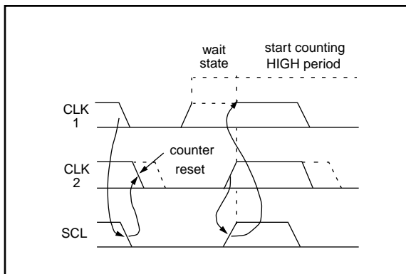
FIGURE 11-17: CLOCK SYNCHRONIZATION
