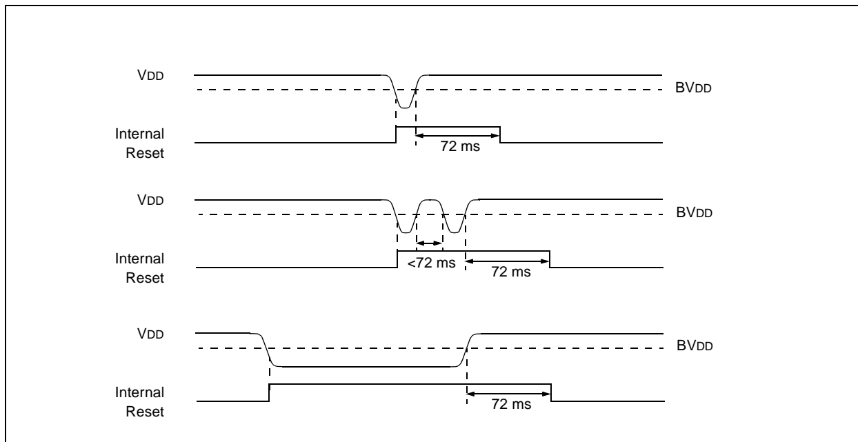
FIGURE 10-7: BROWN-OUT SITUATIONS
