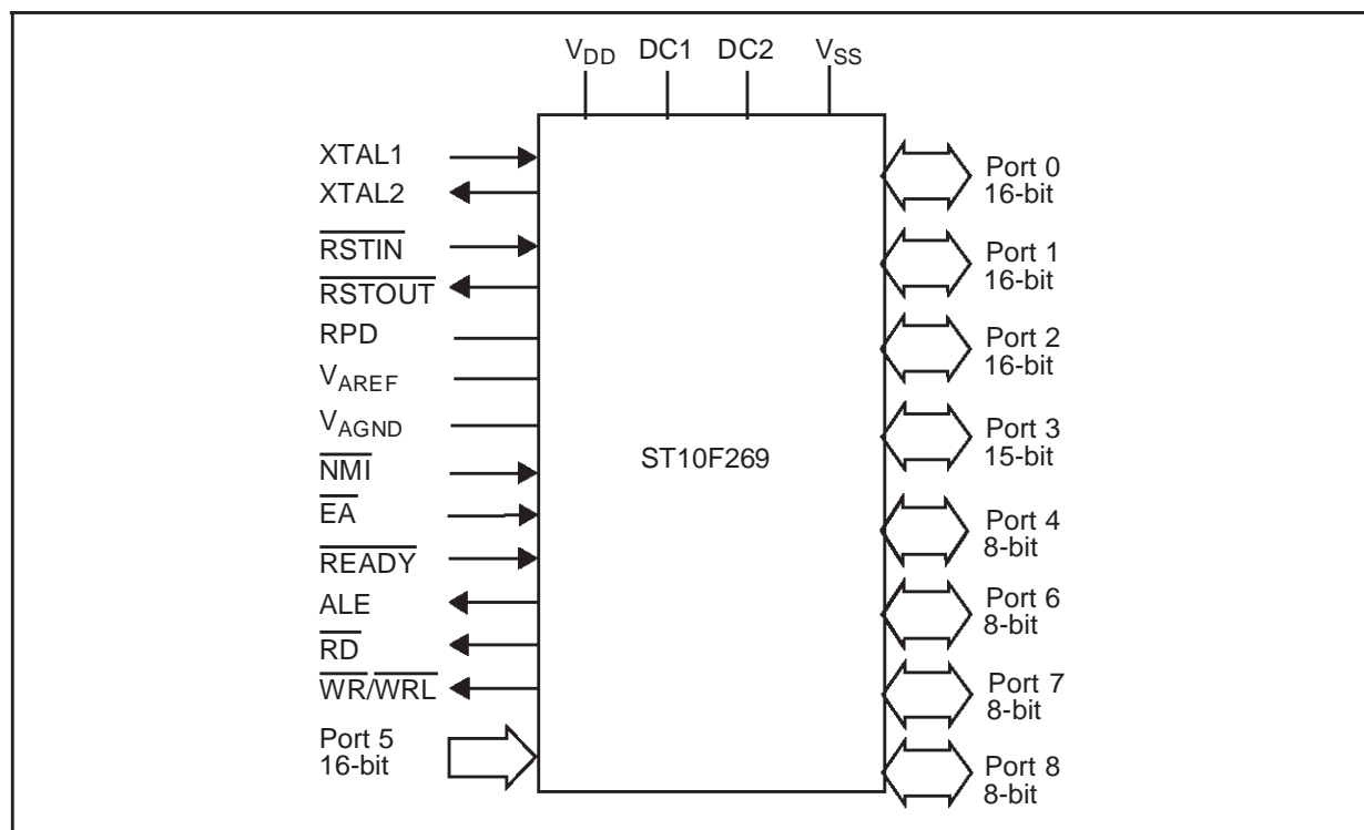
Figure 1 : Logic Symbol
