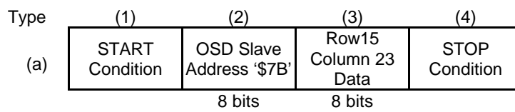
Figure 9: Access Register Write Operation
