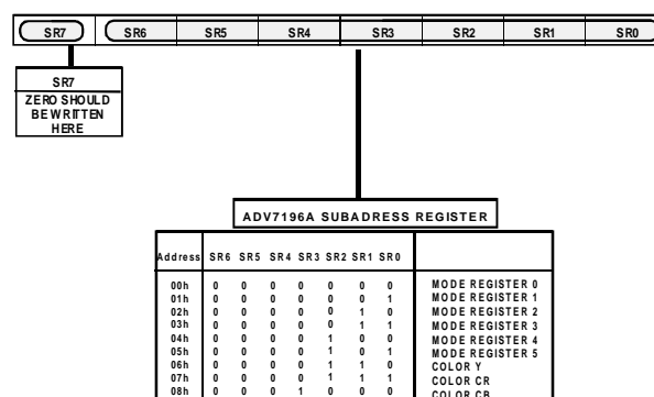
Fig xx. ADV7196A Subaddress Registers in HDTV Mode
