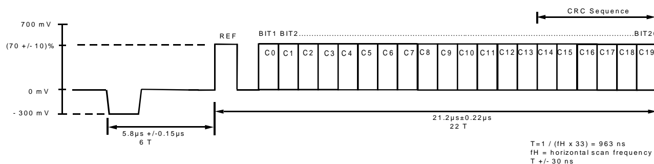
Fig xx. CGMS Waveform
