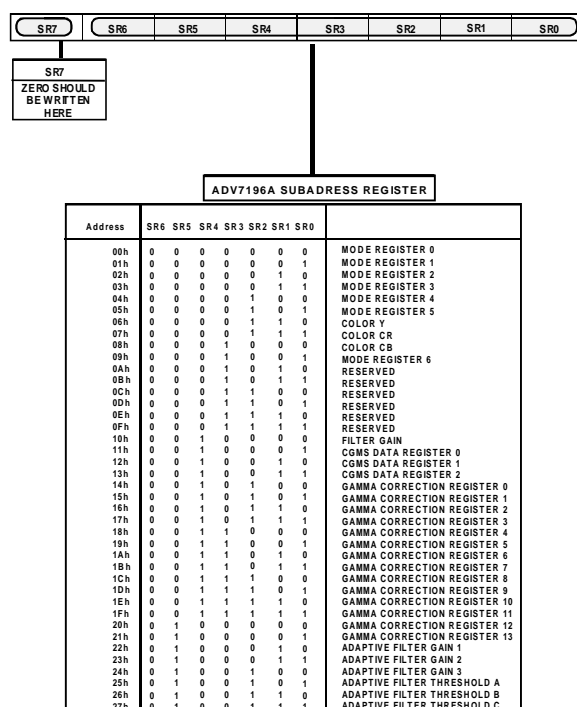
Fig xx. ADV7196A Subaddress Registers in Progressive Scan Mode
