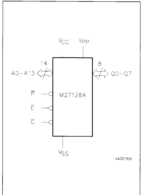
Figure 1. Logic Diagram
