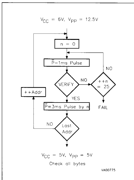
Figure 7. Programming Flowchart
