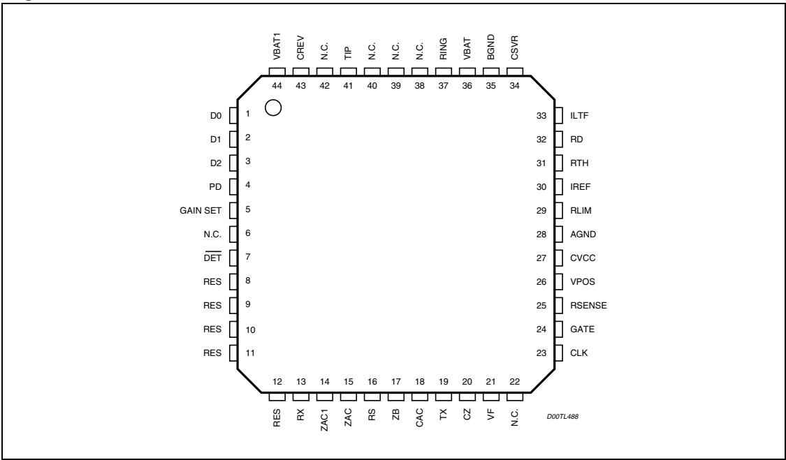
Figure 2. Pin connection
