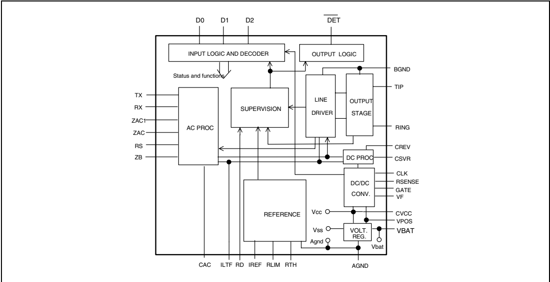
Figure 1. Block diagram
