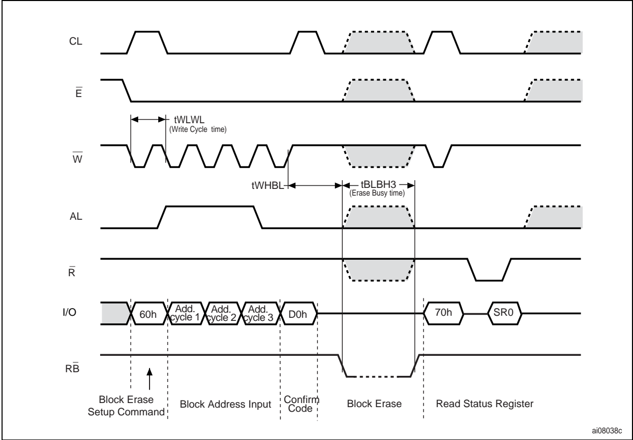
Figure 29. Block Erase AC Waveform
