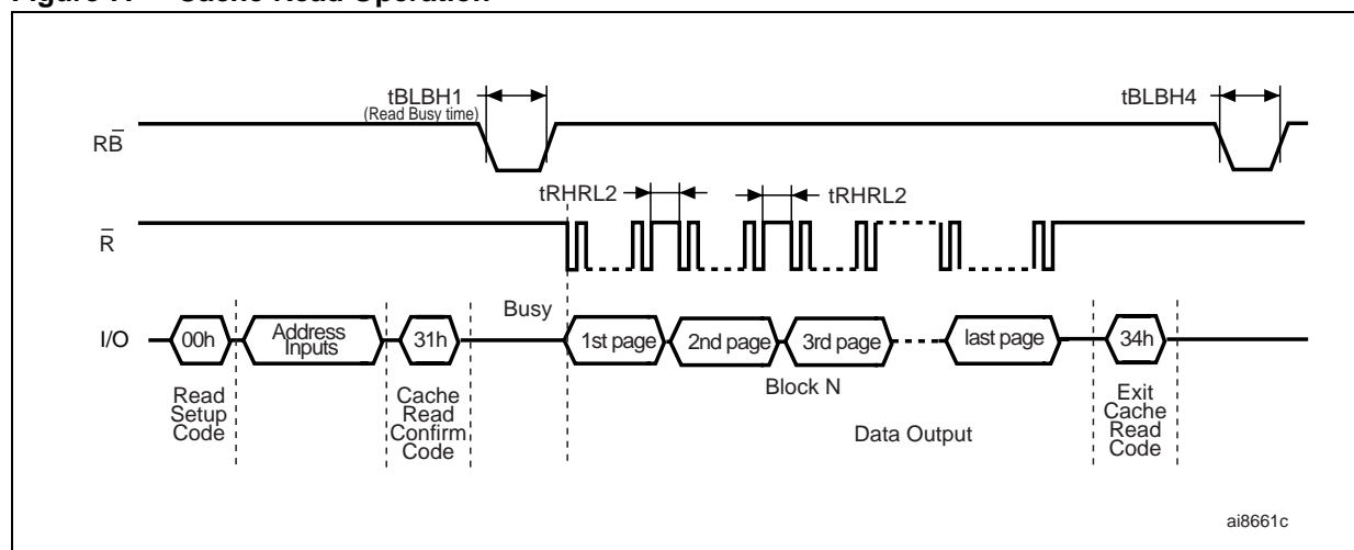
Figure 7. Cache Read Operation
