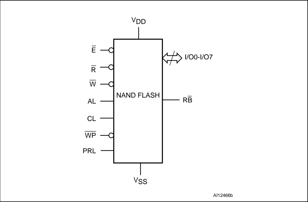
Figure 2. Logic Diagram
