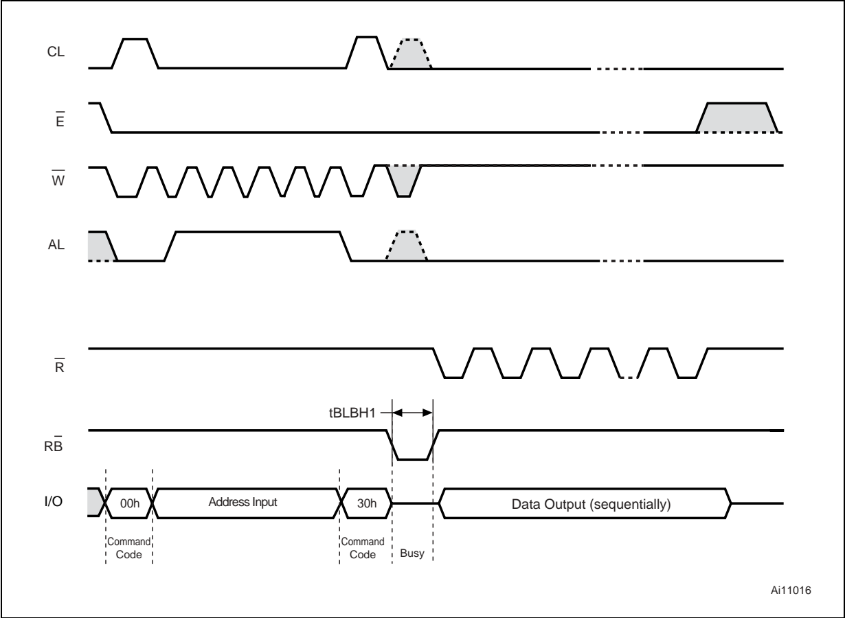
Figure 5. Read Operations
