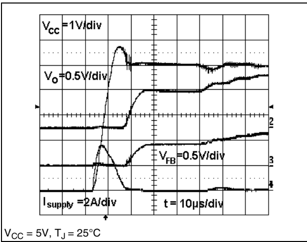
Figure 20. Start-Up transient
