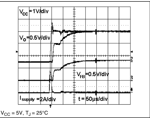
Figure 21. Start-Up transient
