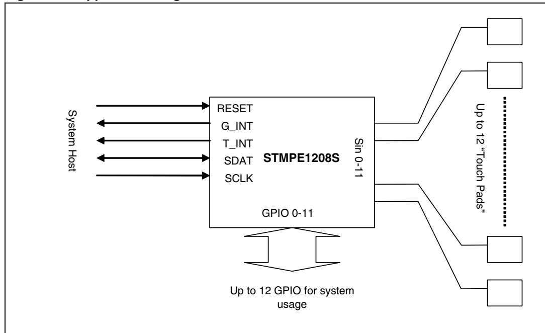
Figure 3. Application diagram
