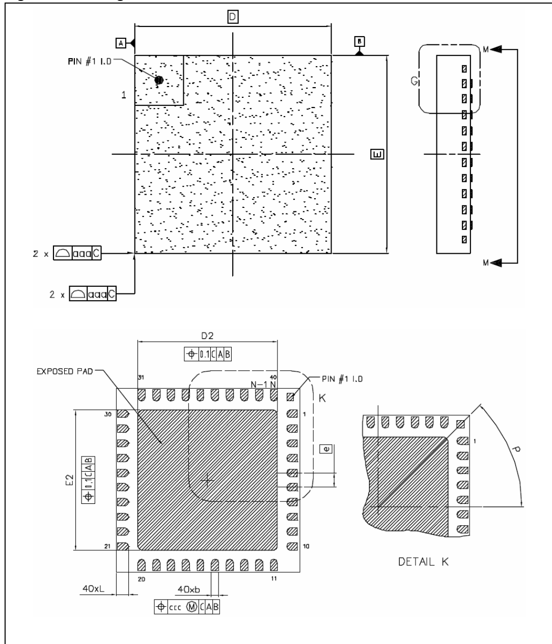
Figure 5. Package dimensions
