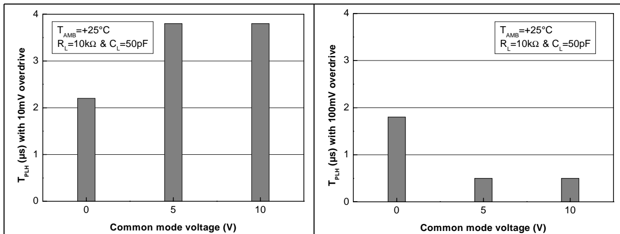
Figure 7. T_{PLH} vs V_{icm} at V_{CC} = 10V and 10mV overdrive Figure 8. T_{PLH} vs V_{icm} at V_{CC} = 10V and 100mV overdrive
