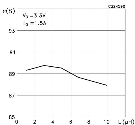
Figure 8. Efficiency vs inductor
