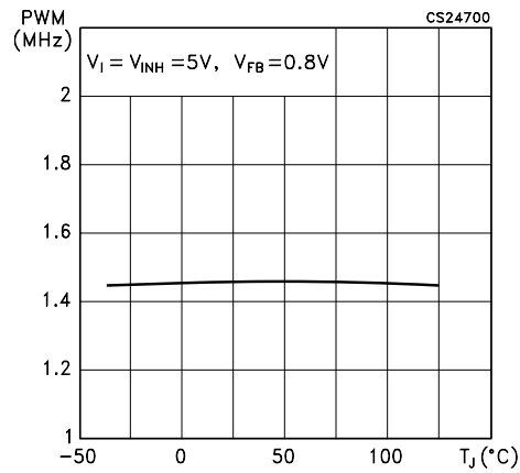
Figure 19. PWM Switching Frequency vs temperature
