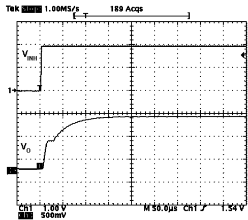
Figure 22. Inhibit transient
