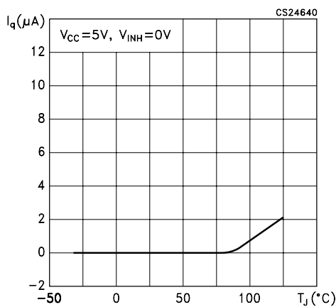
Figure 13. Quiescent current vs temperature
