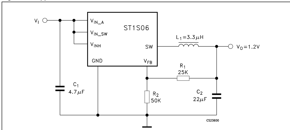
Figure 24. Application circuit
