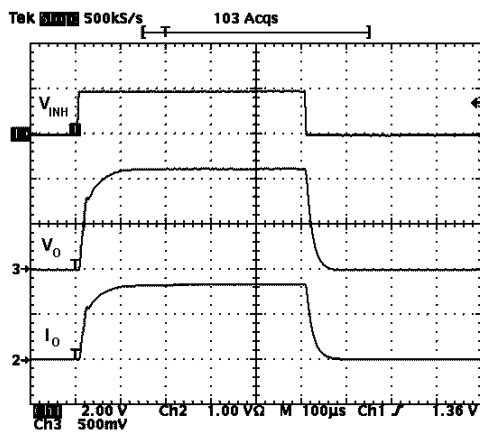
Figure 23. Inhibit transient
