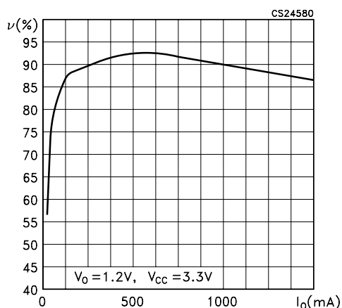
Figure 5. Efficiency vs output current
