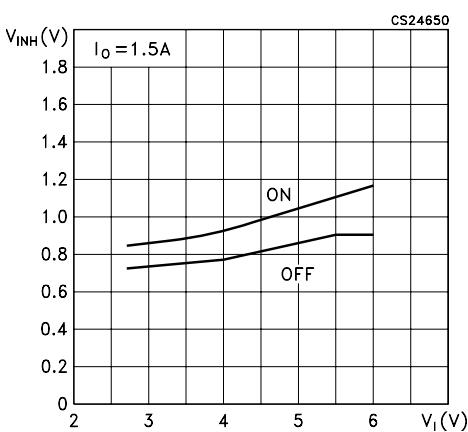
Figure 14. Inhibit voltage vs input voltage
