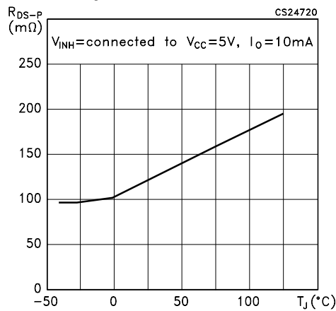
Figure 21. PMOS Switch on resistance vs temperature
