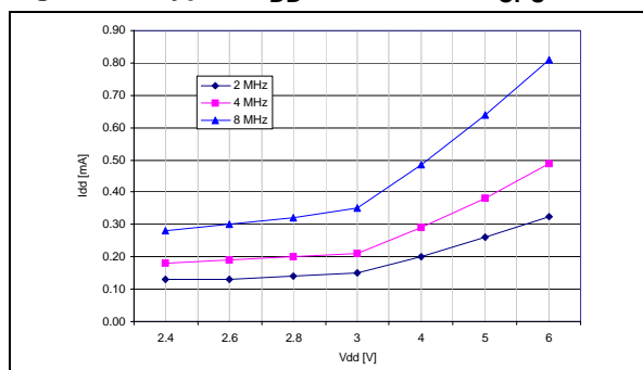
Figure 42. Typical I_{DD} in WAIT vs. f_{CPU}
