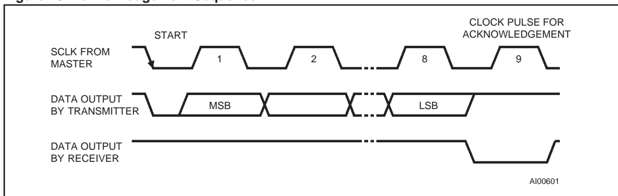
Figure 10. Acknowledgement Sequence
