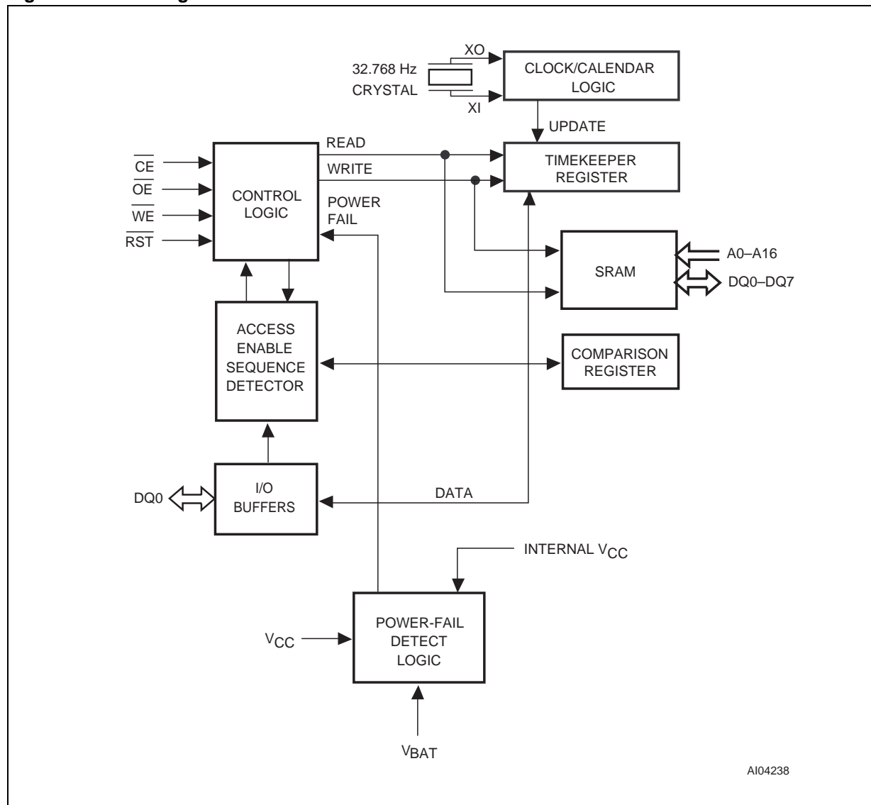
Figure 4. Block Diagram
