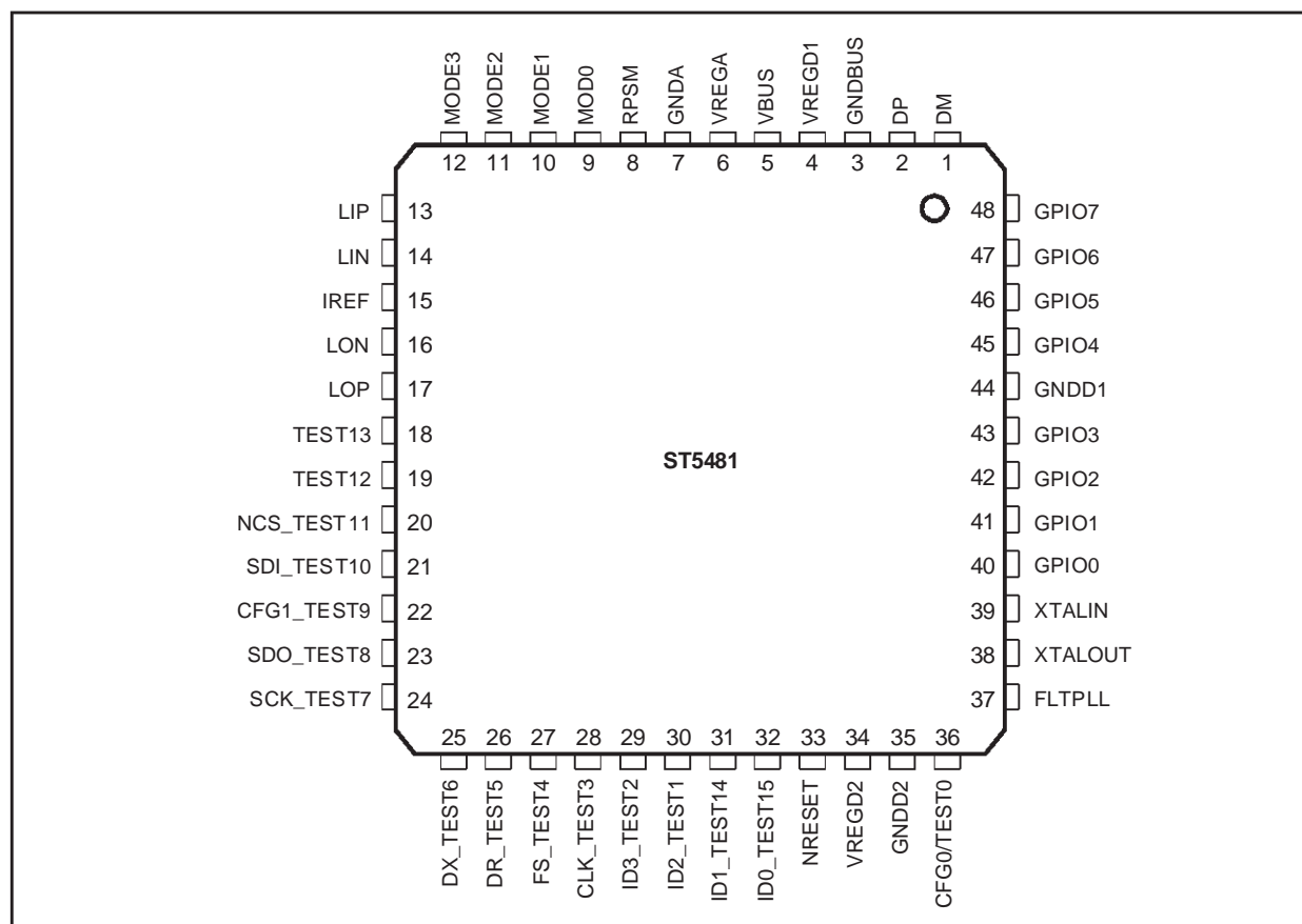
Figure 1 : Pin-out Synoptic
