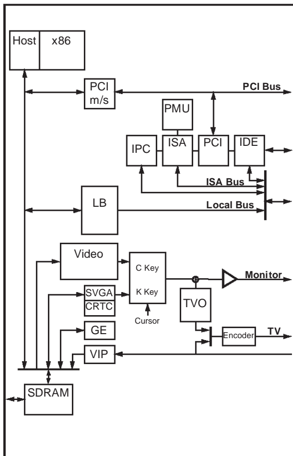
Figure 0-1. Logic Diagram
