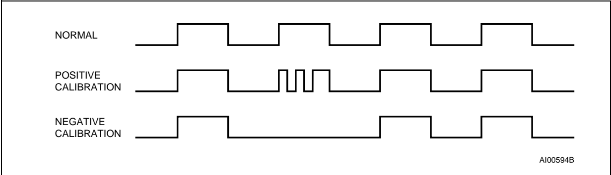
Figure 17. Clock Calibration
