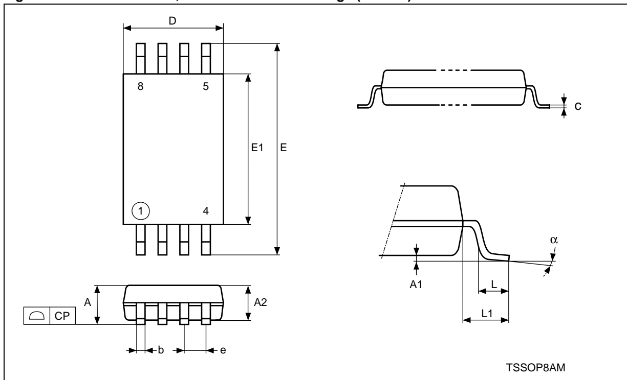
Figure 14. TSSOP8 – 8-lead, Thin Shrink Small Package (3x3mm) Outline
