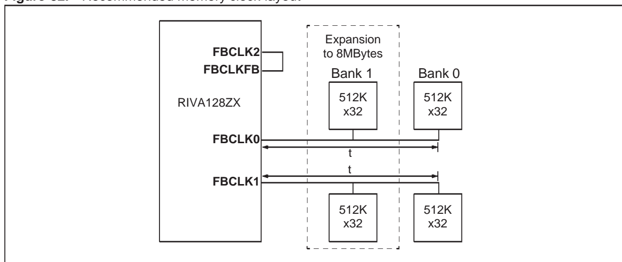
Figure 32. Recommended memory clock layout
