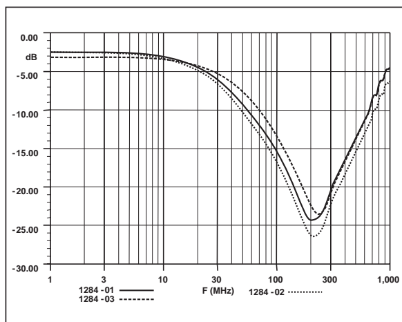
Fig. A2: Typical frequency response curve for data and strobe signals.
