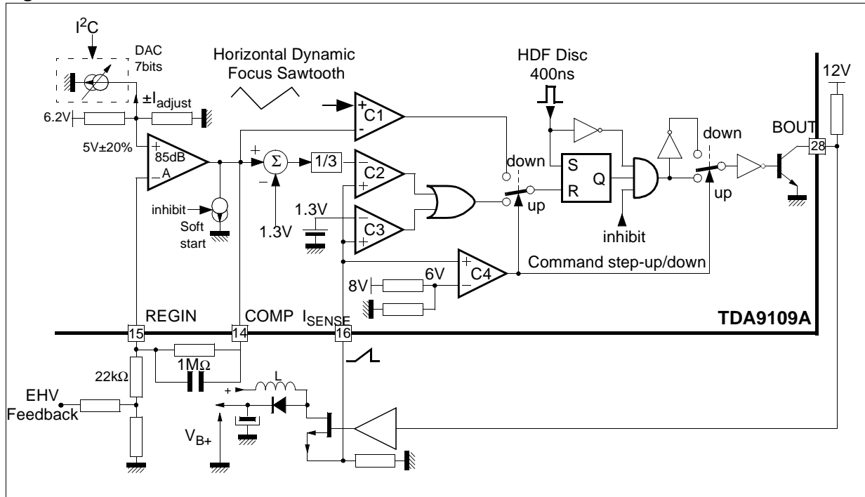
Figure 18. DC/DC Convertor
