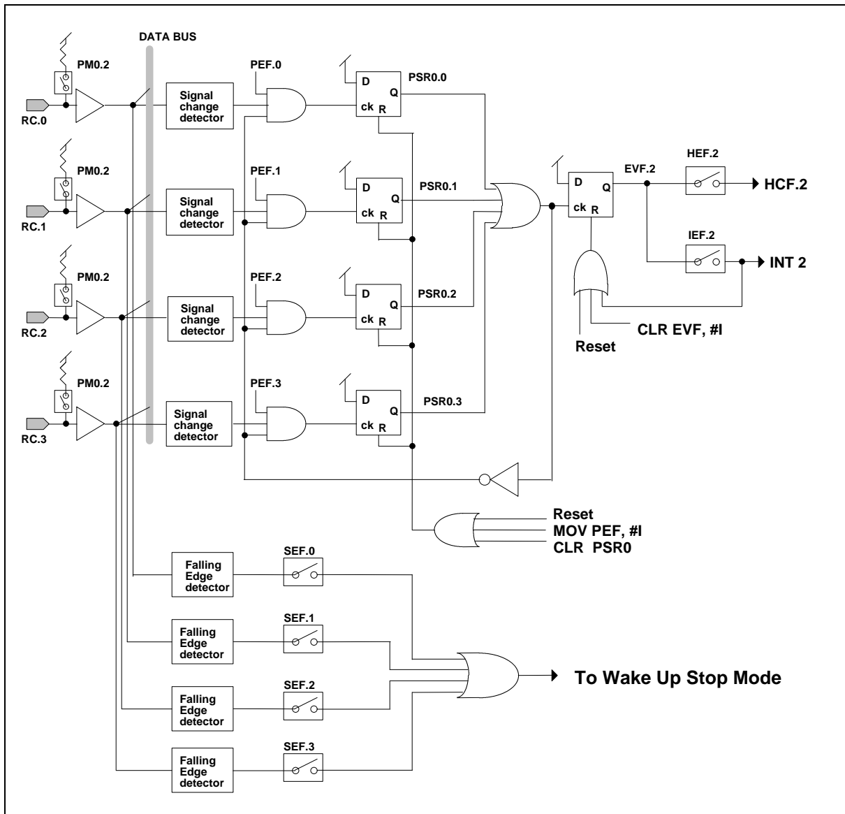
Figure 6-12 Architecture of Input Ports RC
