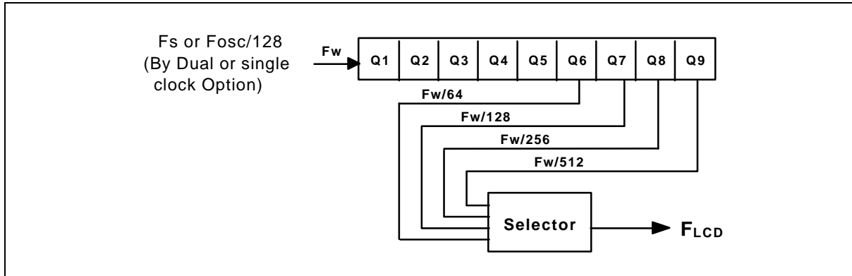
Figure 6-14 LCD alternating frequency ( F_{LCD} ) circuit diagram
