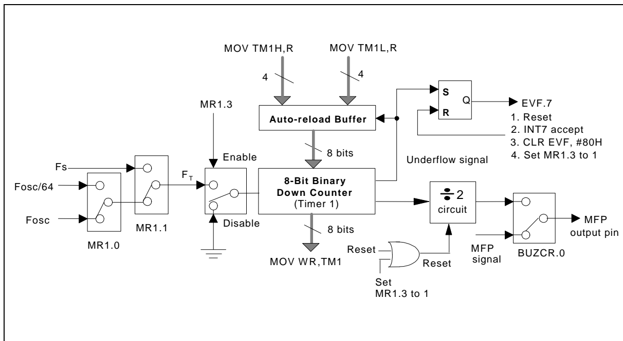
Figure 6-7 Organization of Timer 1
