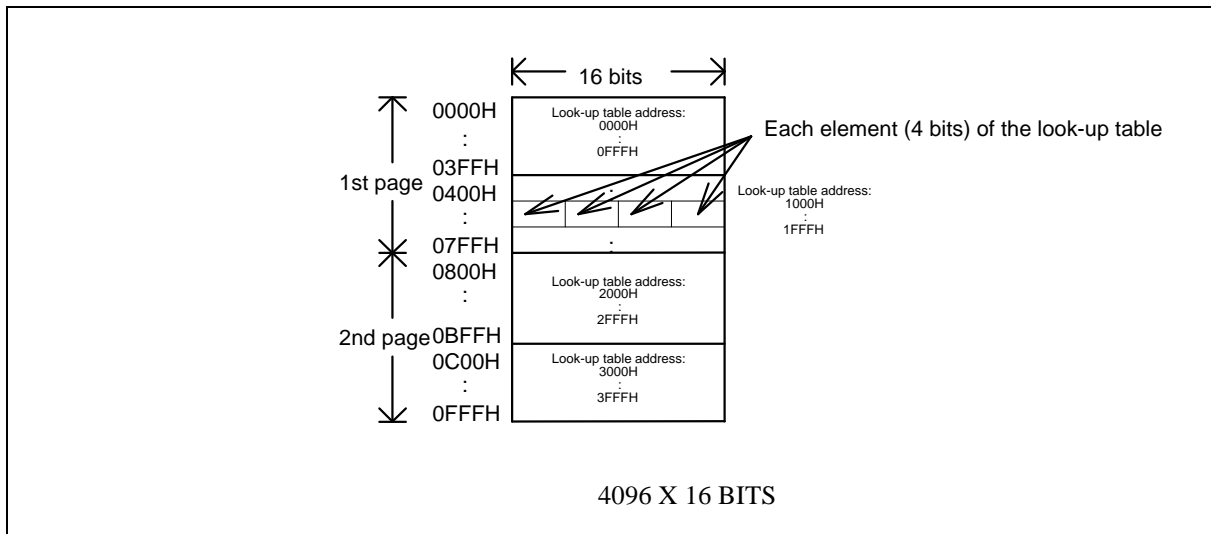
Figure 6-1 Program Memory Organization
