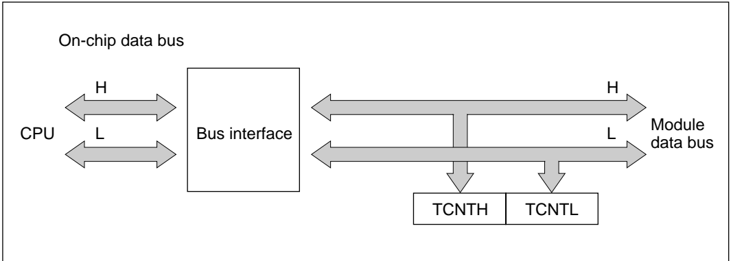
Figure 8-6 Access to Timer Counter (CPU Writes to TCNT, Word)
