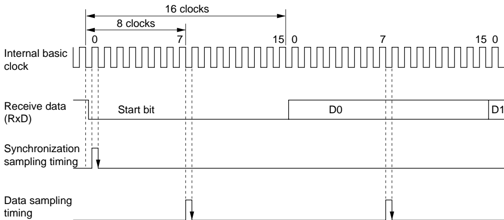
Figure 12-21 Receive Data Sampling Timing in Asynchronous Mode
