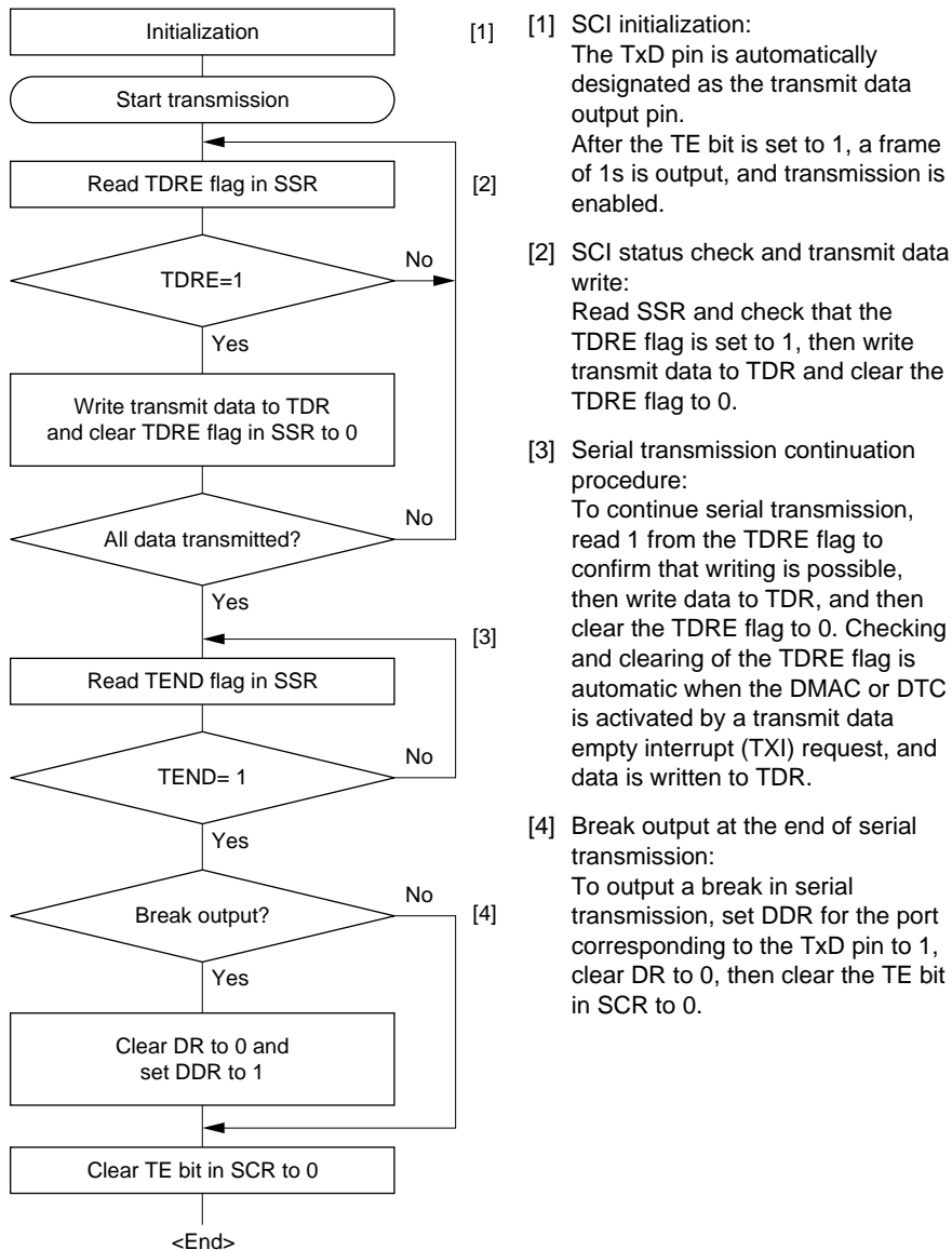
Figure 13-5 Sample Serial Transmission Flowchart
