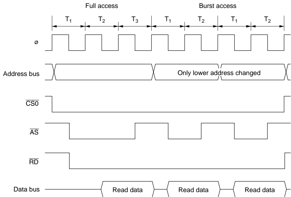
Figure 6-30 (a) Example of Burst ROM Access Timing (When AST0 = BRSTS1 = 1 )
