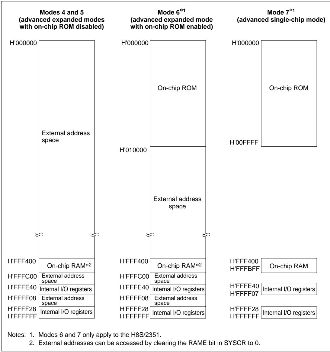
Figure 3-1 Memory Map in Each Operating Mode (cont)
