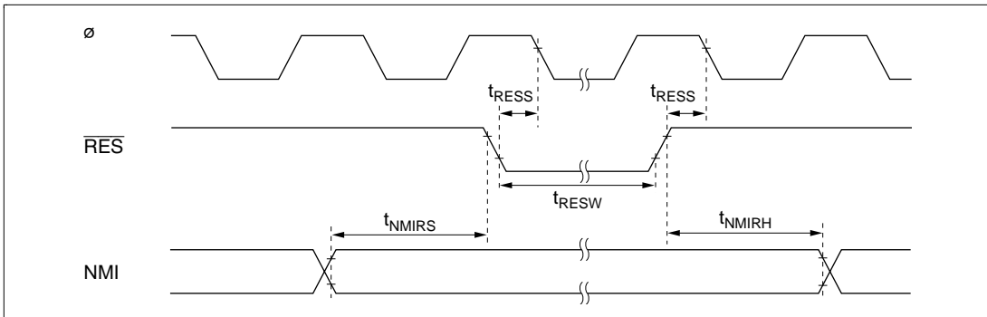
Figure 21-6 Reset Input Timing
