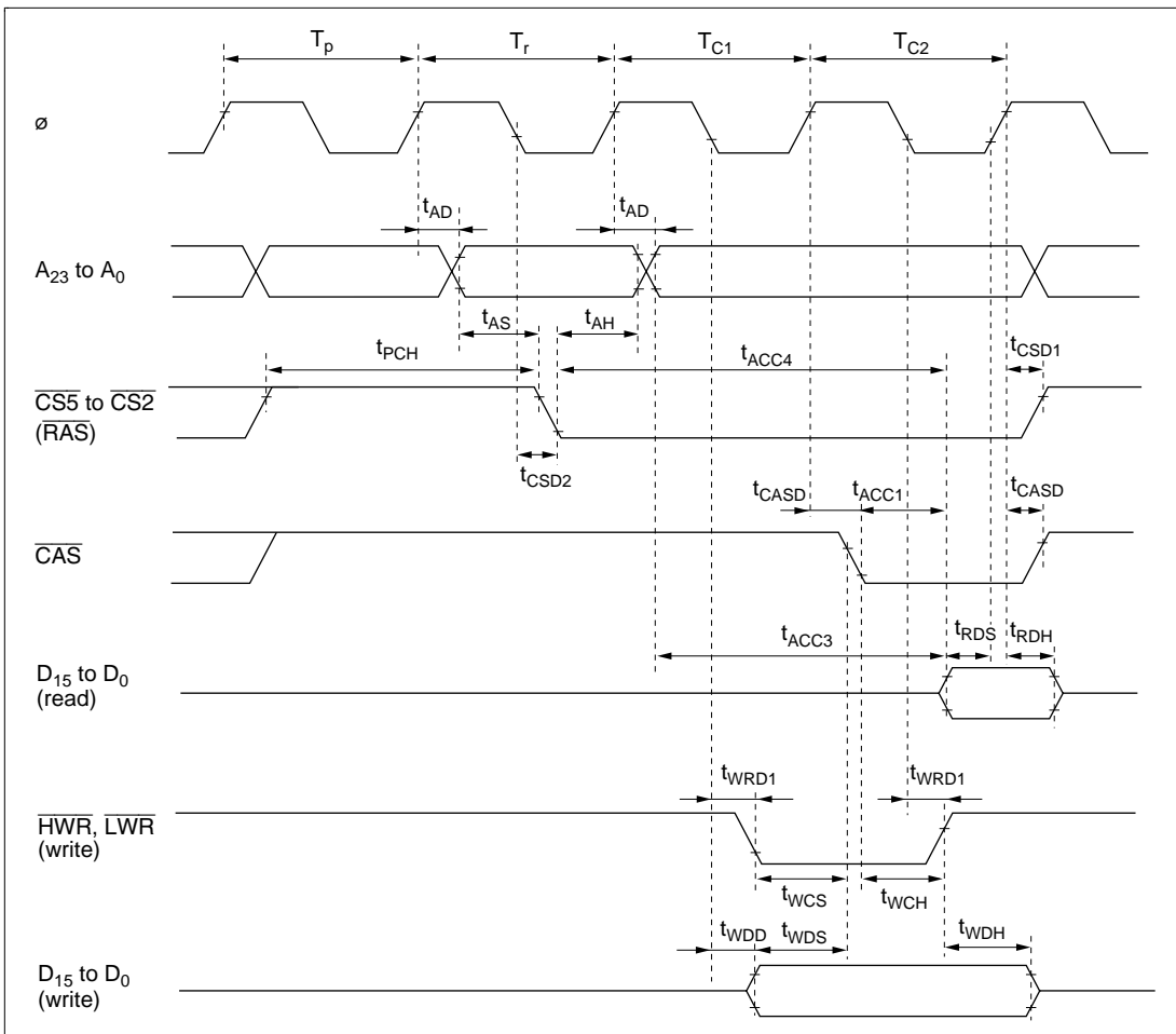
Figure 21-11 DRAM Bus Timing
