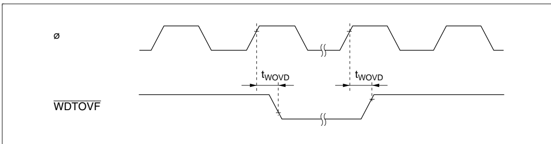
Figure 21-26 WDT Output Timing
