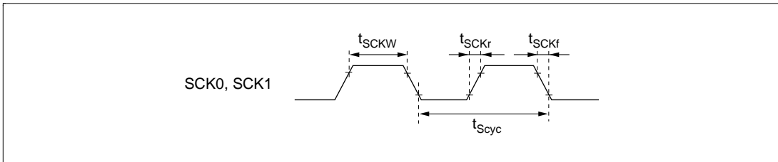
Figure 21-27 SCK Clock Input Timing
