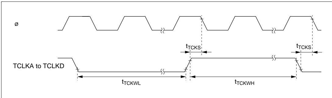
Figure 21-25 TPU Clock Input Timing
