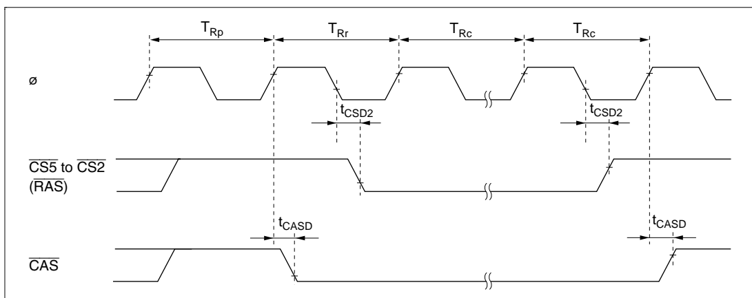
Figure 21-13 Self-Refresh Timing
