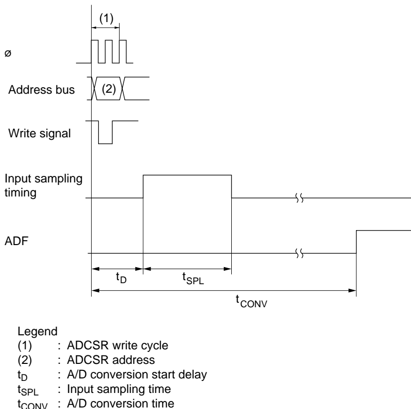
Figure 15-5 A/D Conversion Timing
