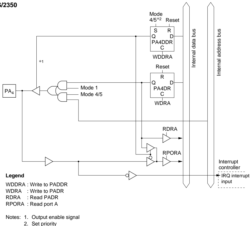
Figure C-7 (b-2) H8S/2350 Port A Block Diagram (Pin PA 4 )
