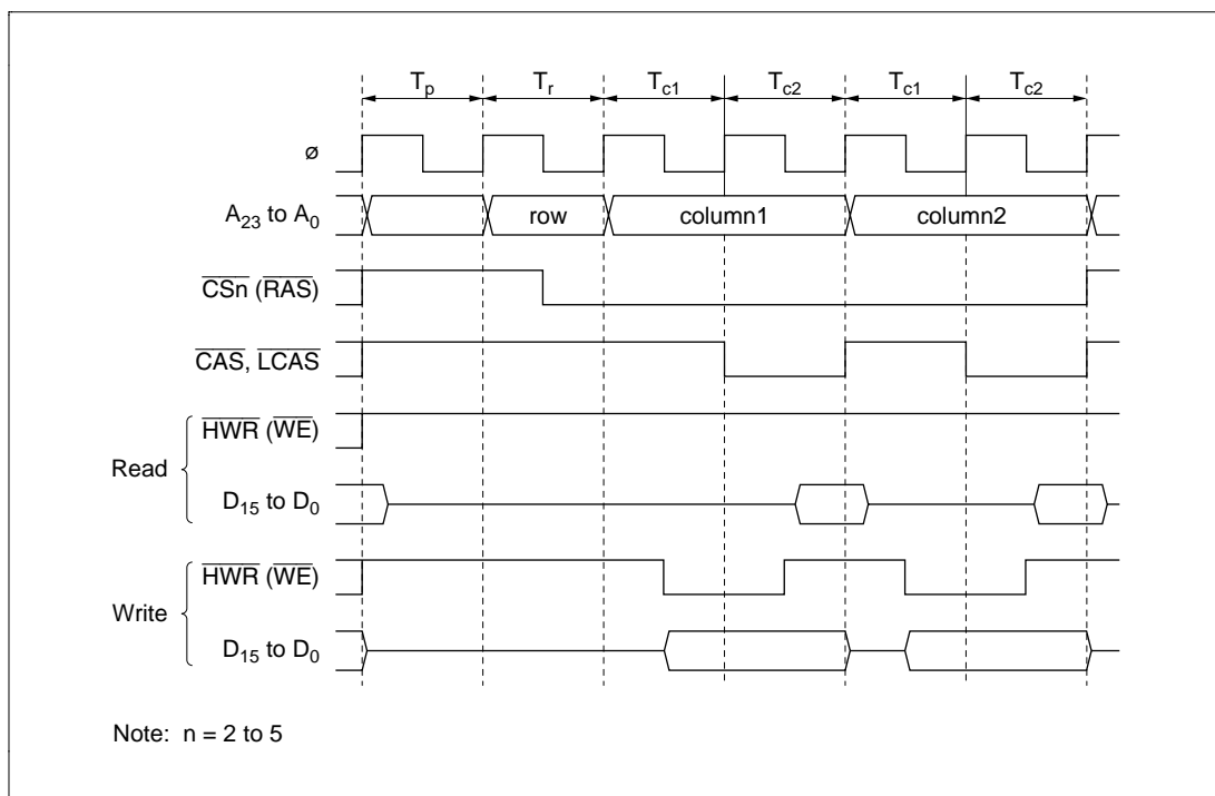
Figure 6-20 Operation Timing in Fast Page Mode (2-WE System)
