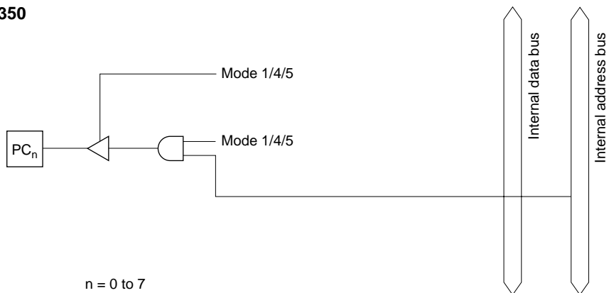
Figure C-9 (b) H8S/2350 Port C Block Diagram (Pin PC_n )
