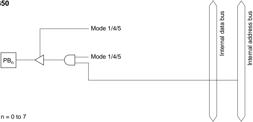
Figure C-8 (b) H8S/2350 Port B Block Diagram (Pin PB_n )
