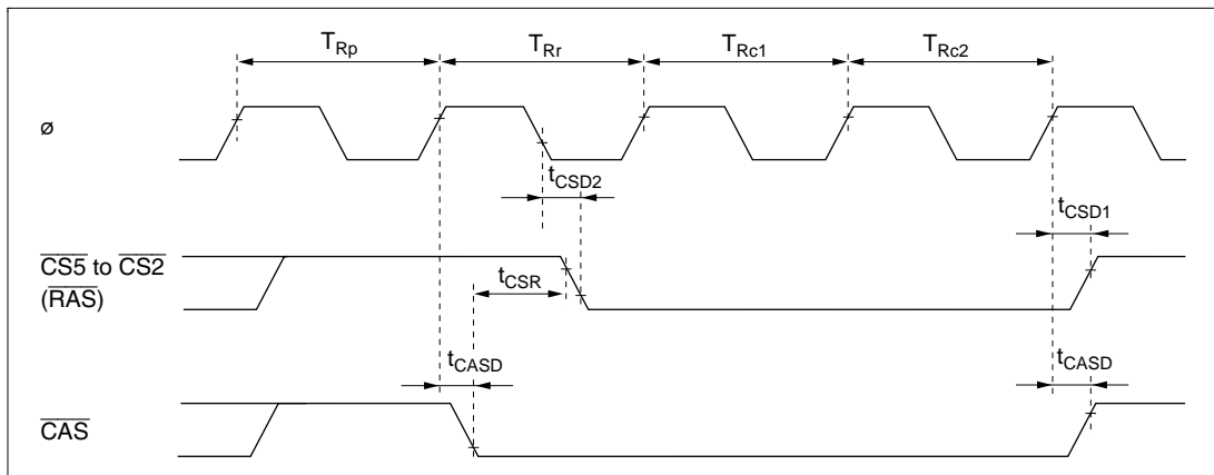
Figure 21-12 CAS-Before-RAS Refresh Timing
