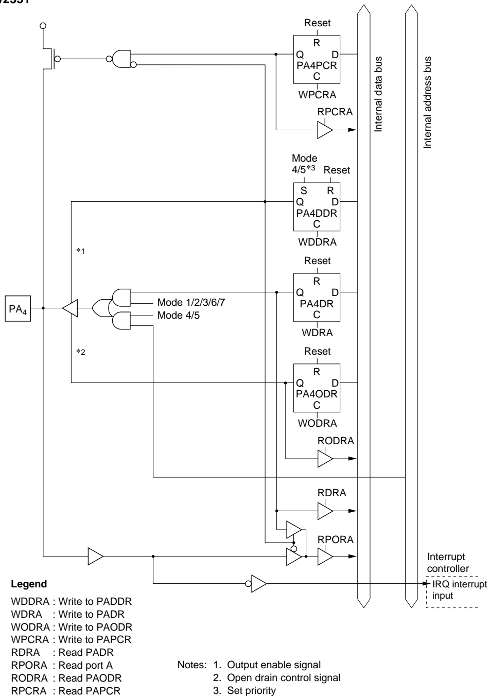
Figure C-7 (b-1) H8S/2351 Port A Block Diagram (Pin PA 4 )
