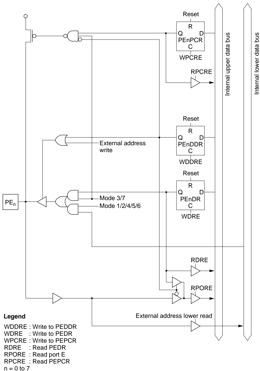
Figure C-11 Port E Block Diagram (Pin PE n )
