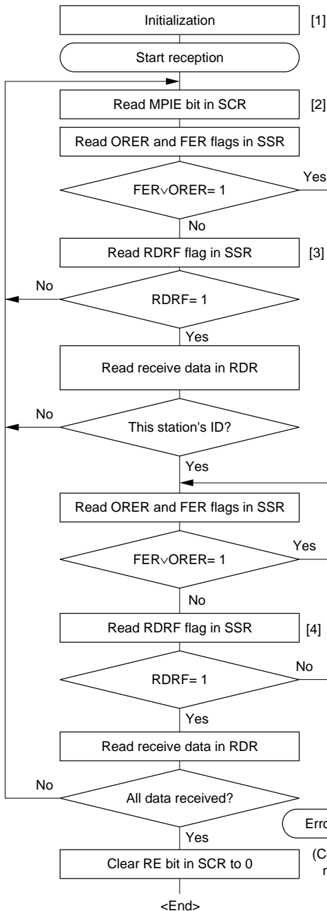
Figure 12-12 Sample Multiprocessor Serial Reception Flowchart
