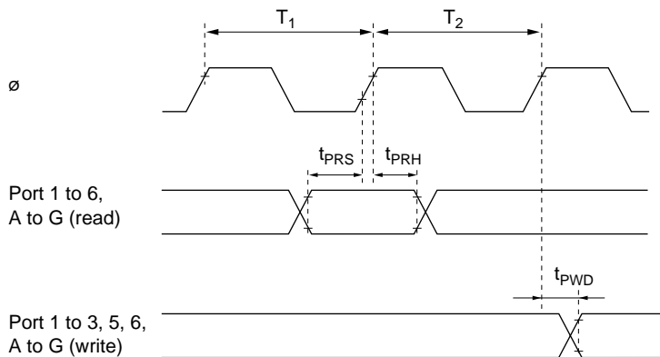
Figure 20-14 I/O Port Input/Output Timing
