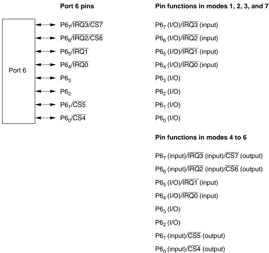
Figure 8-6 Port 6 Pin Functions
