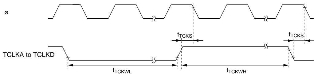
Figure 20-16 TPU Clock Input Timing
