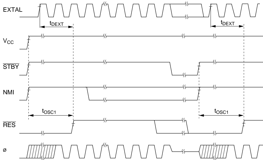
Figure 20-5 Oscillator Settling Timing
