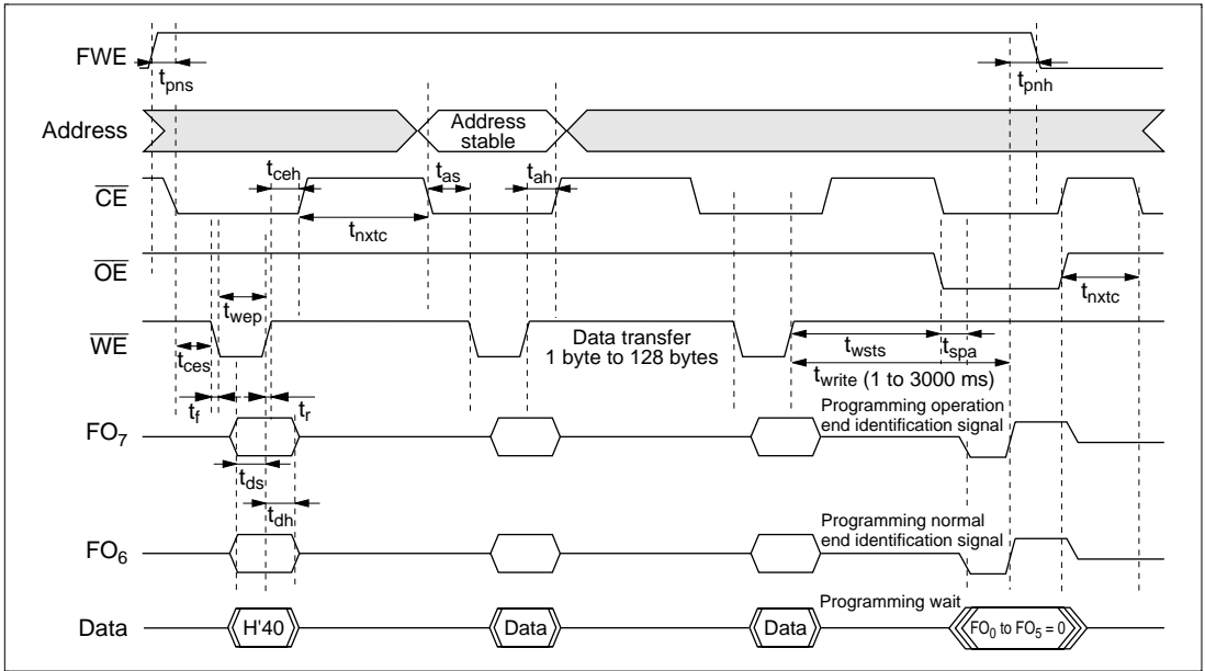
Figure 17.31 Auto-Program Mode Timing Waveforms
