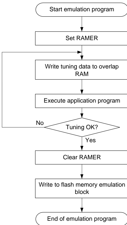
Figure 17.24 Flowchart for Flash Memory Emulation in RAM
