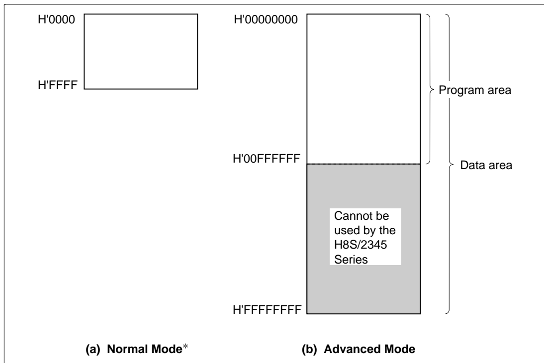
Figure 2.6 Memory Map
