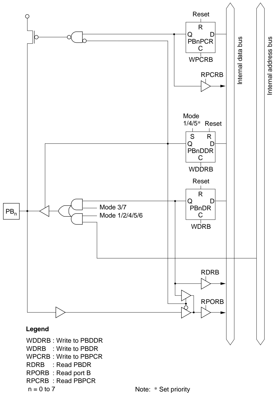
Figure C.6 Port B Block Diagram (Pin PB n )
