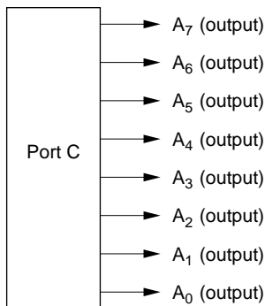
Figure 8.14 Port C Pin Functions (Modes 1, 4, and 5)*
