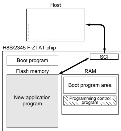
Figure 17.9 Boot Mode
