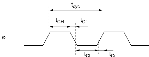
Figure 20.7 System Clock Timing
