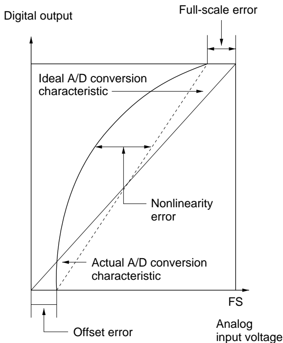
Figure 14.10 A/D Conversion Precision Definitions (2)
