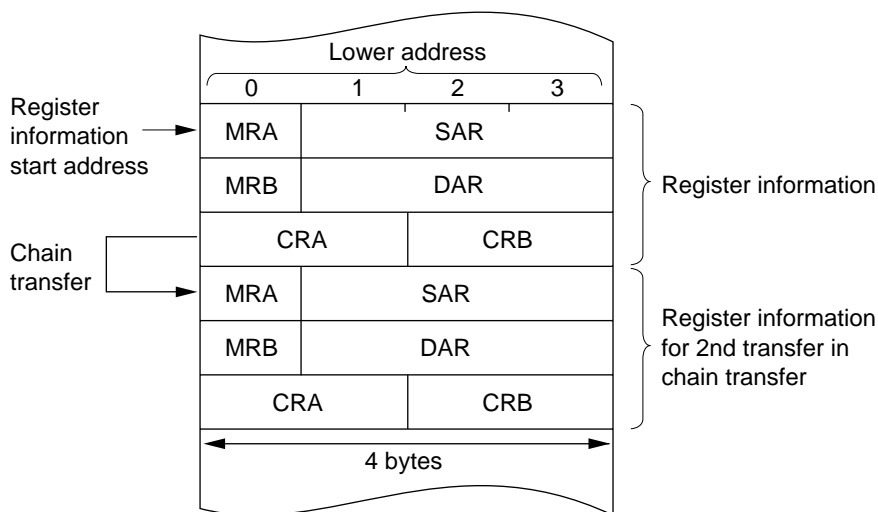
Figure 7.5 Location of Register Information in Address Space
