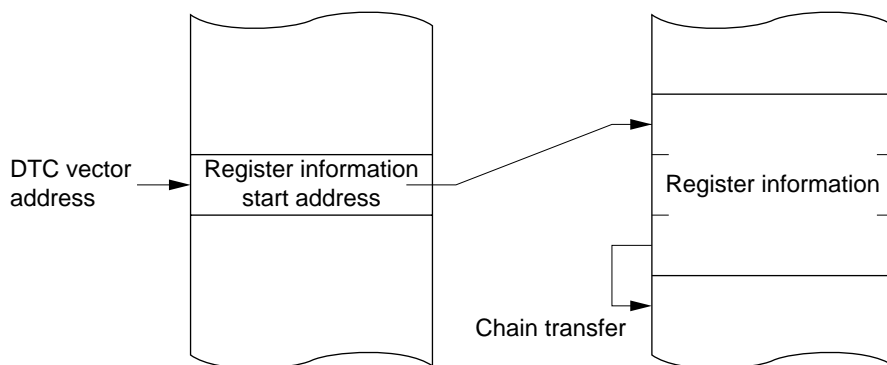
Figure 7.4 Correspondence between DTC Vector Address and Register Information
