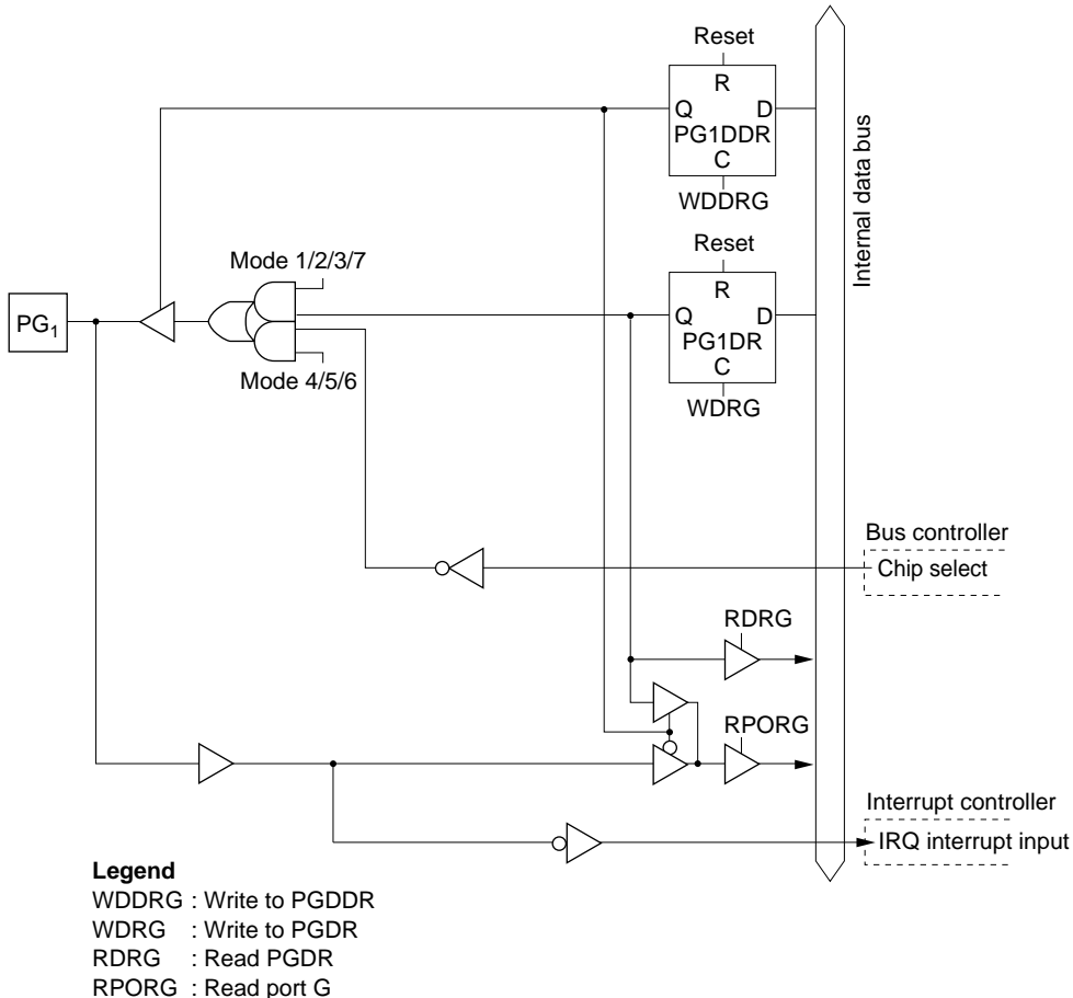
Figure C.11 (b) Port G Block Diagram (Pin PG 1 )
